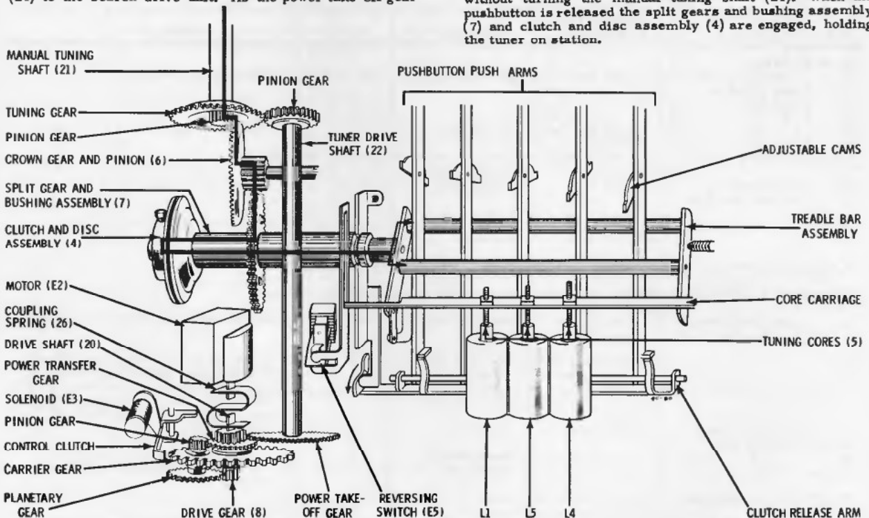
FIGURE 2. MANUAL TUNING
