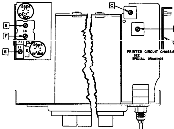
PARTS LAYOUT — TUBE VIEW
