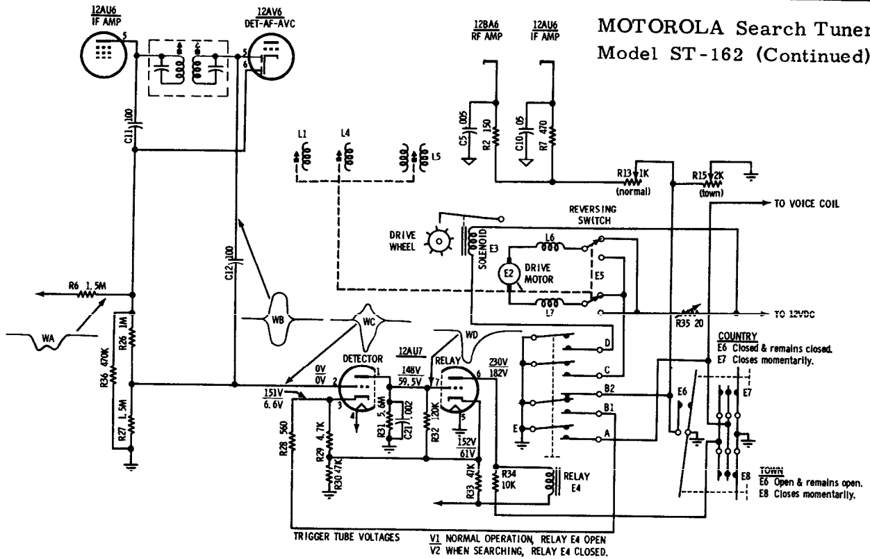
FIGURE 7. FUNCTIONAL SCHEMATIC
