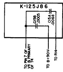
Bullplate
