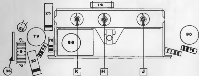
PARTS LAYOUT — TUBE VIEW
