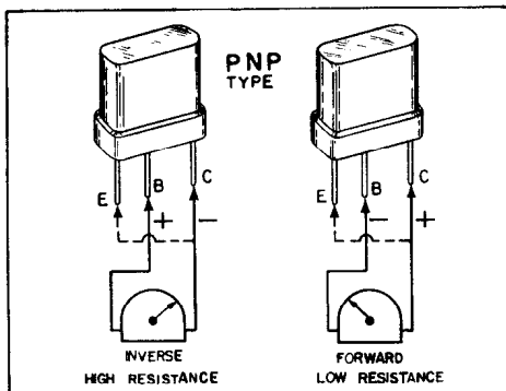
FIGURE 2 - PNP TYPE
