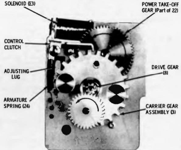
FIGURE 10. CLUTCH ENGAGED
