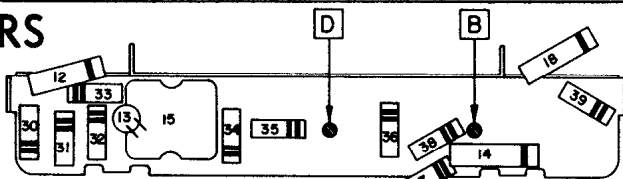
PARTS LAYOUT - CHASSIS VIEW
