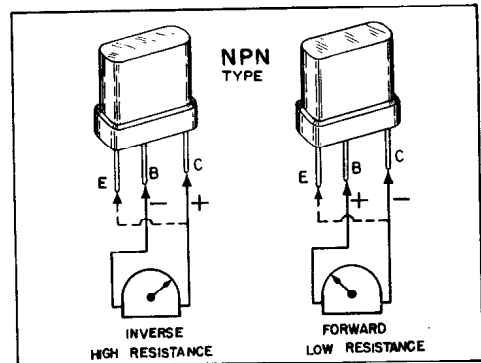
FIGURE 3 - NPN TYPE
