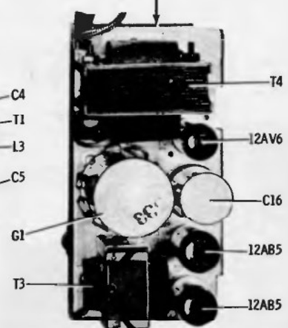
TOP VIEW POWER SUPPLY 841, 842 & 843
