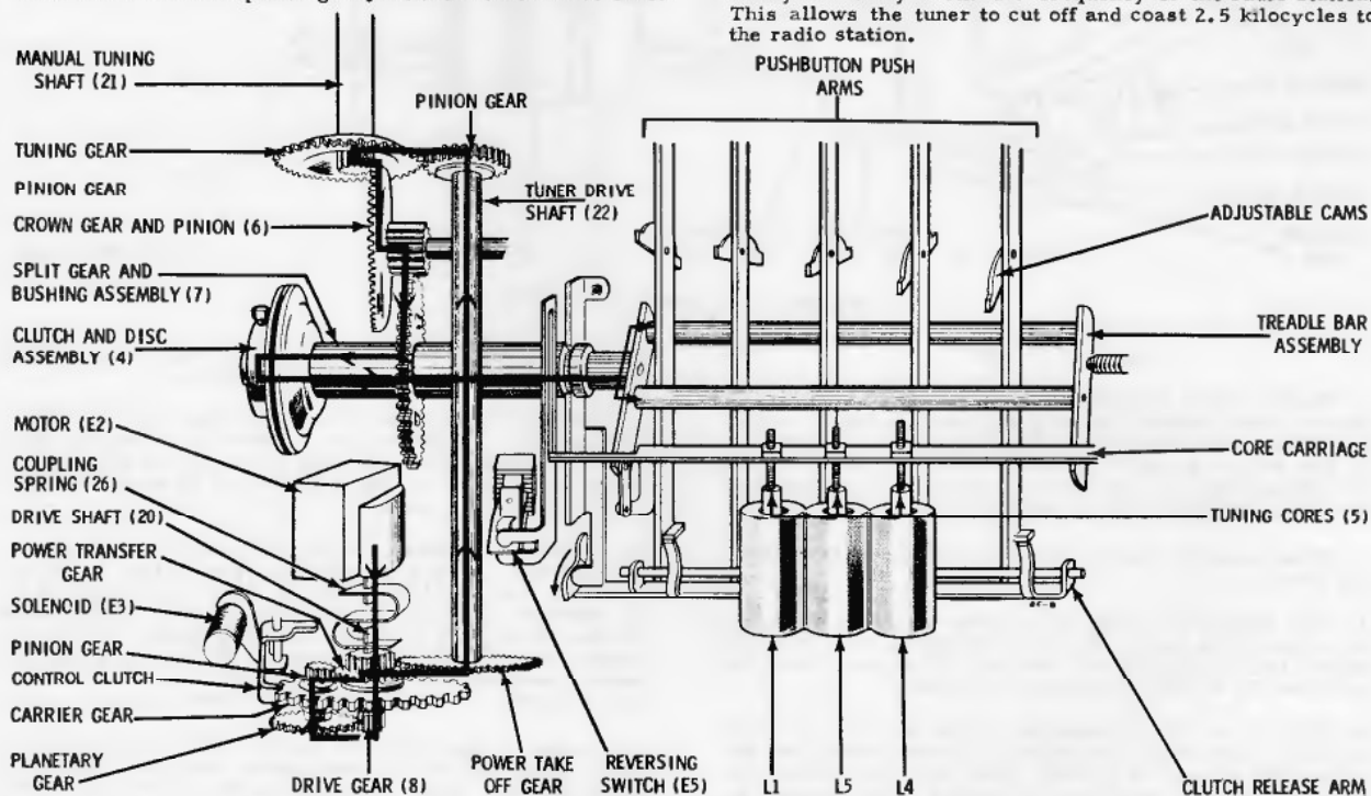
FIGURE 6. SEARCH TUNING
