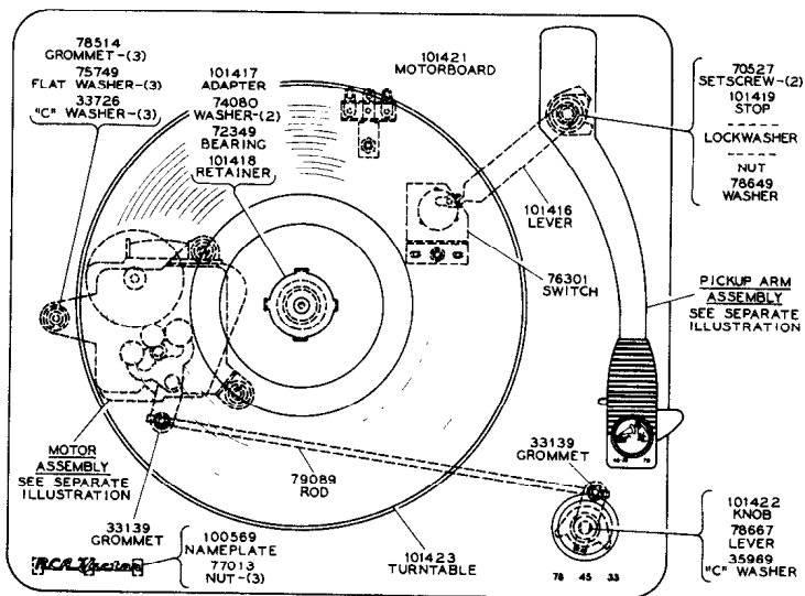
Motorboard Assembly
