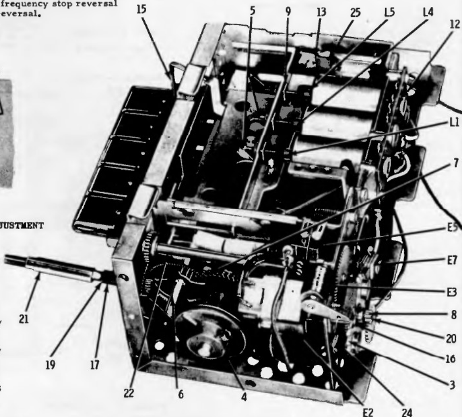
FIGURE 13. TUNER PARTS LOCATIONS
