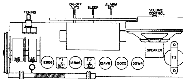
TUBE LAYOUT
