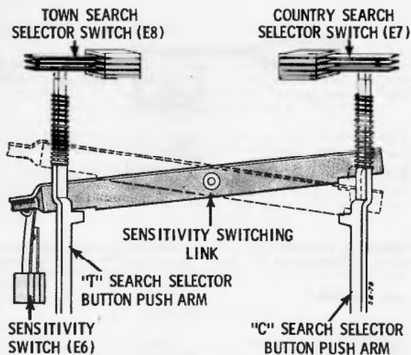
FIGURE 5. SWITCH OPERATIONS
