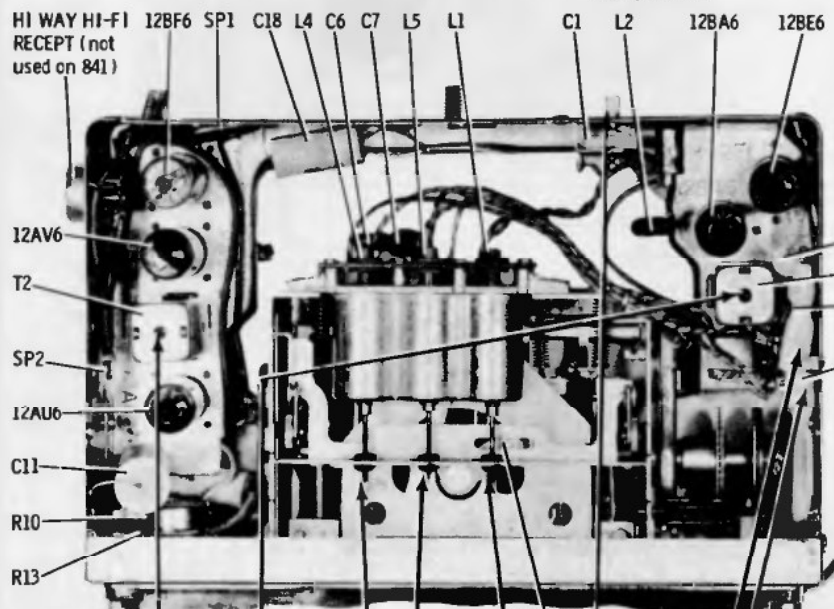
TOP VIEW POWER SUPPLY 841, 842 & 843
