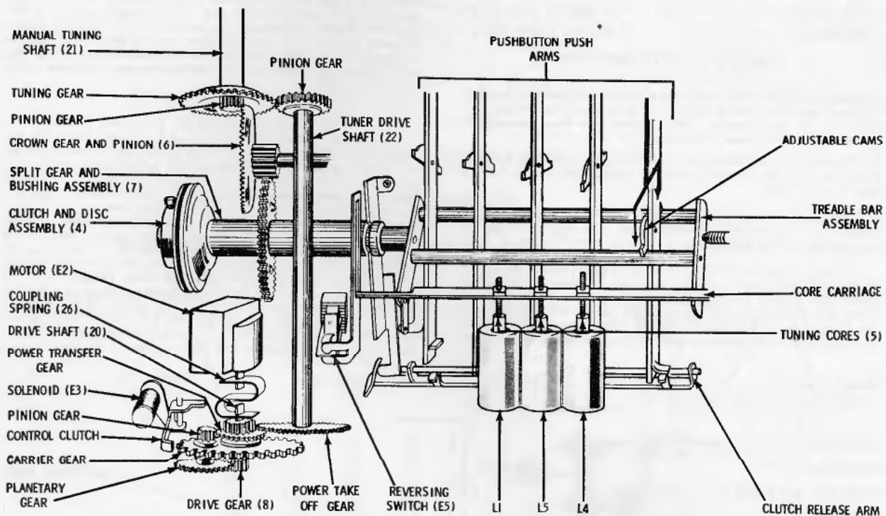
FIGURE 4. PUSHBUTTON TUNING
