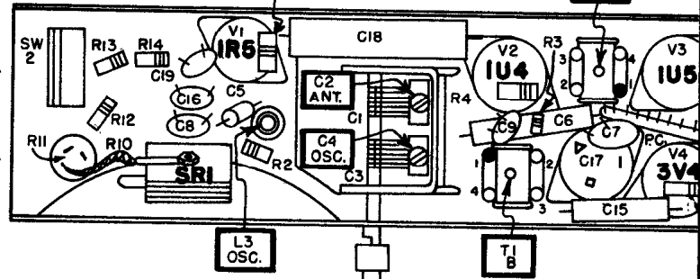
BOTTOM PARTS LAYOUT
