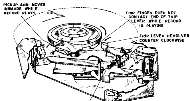
THE TRIP ADJUSTMENT SCREW ON PICKUP ARM LEVER ACTUATES TRIP LEVER
