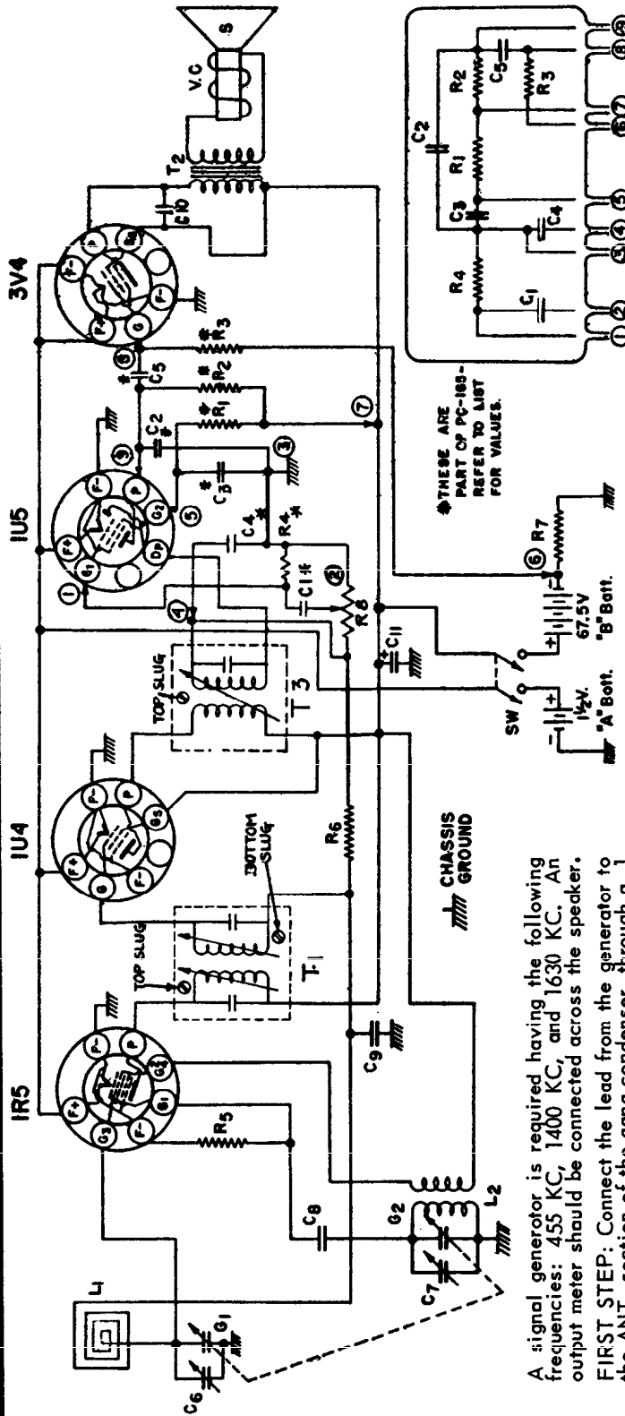
PC-105 WIRING DIAGRAM
