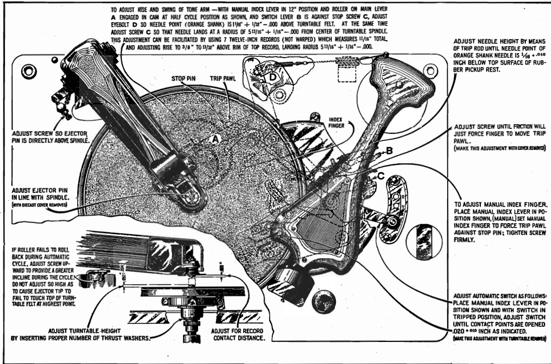
Figure 14—Automatic Record Changer Adjustments
