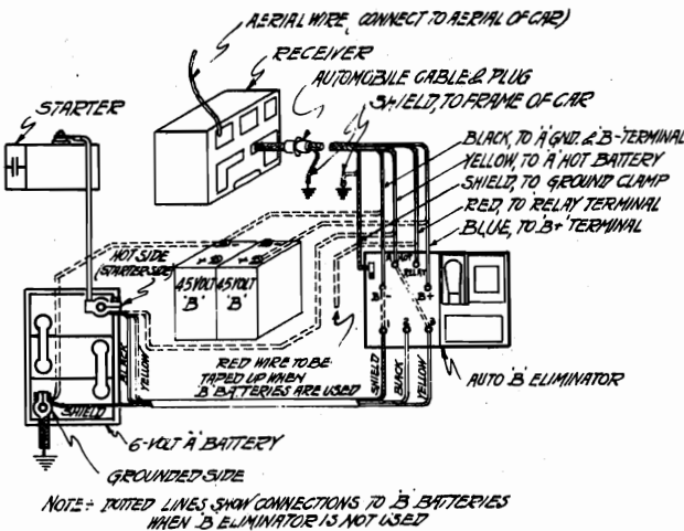
FIG. 2 SKETCH SHOWING CABLE CONNECTIONS TO 'B' ELIMINATOR OR 'B' BATTERIES FOR 6 VOLT A.C. OPERATION
