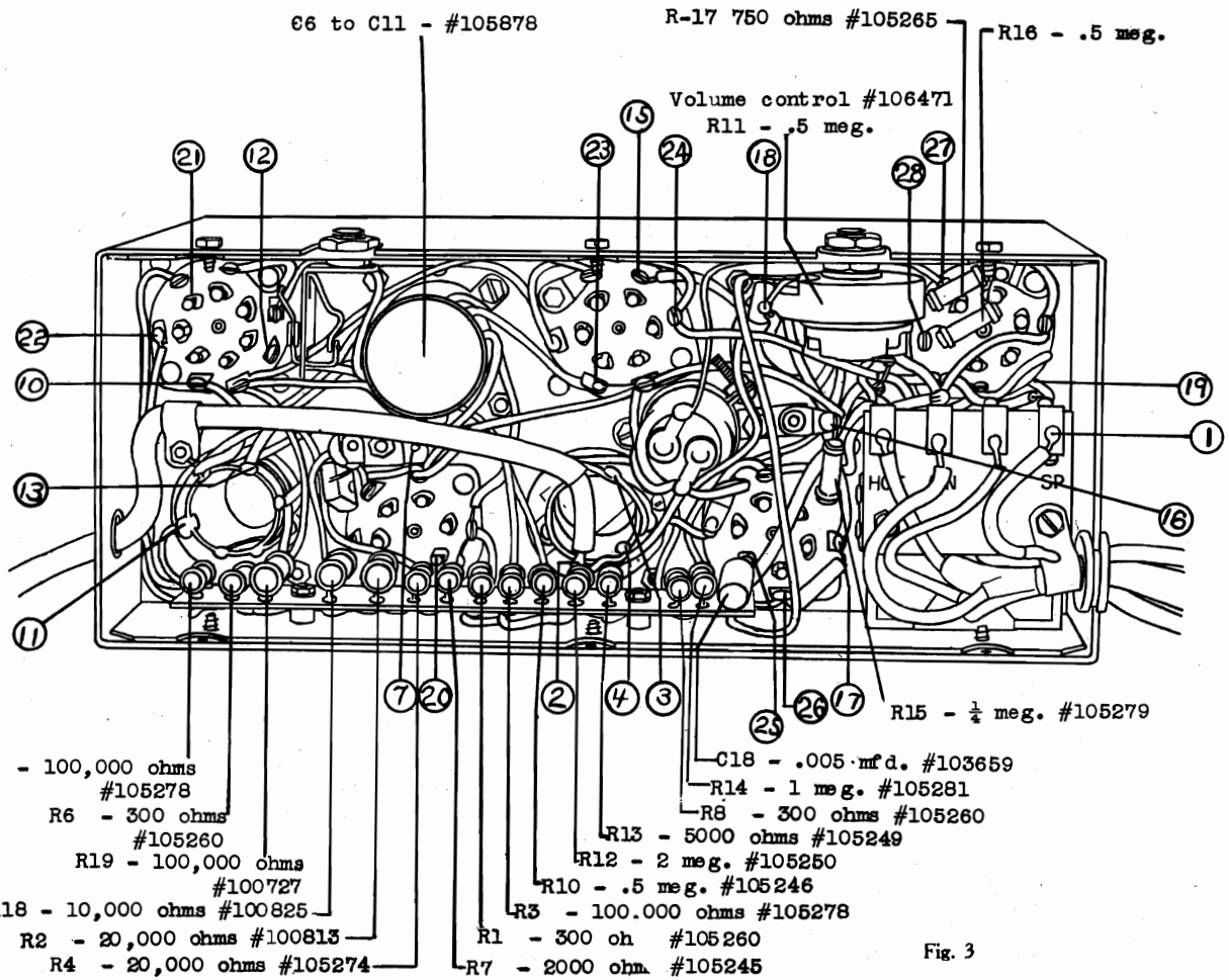
CHASSIS RESISTANCE CHART
