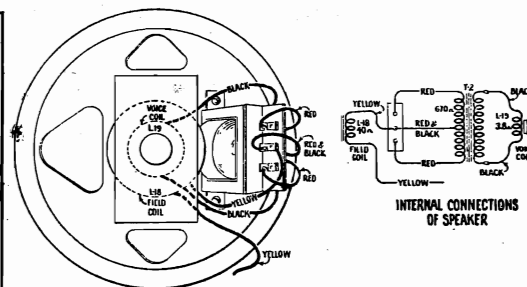
Figure 3—Loudspeaker Wiring
