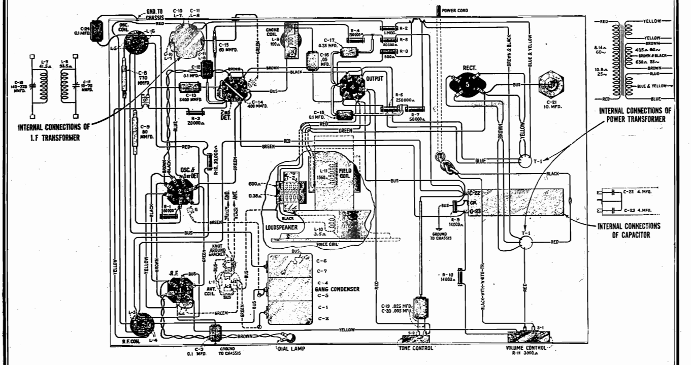
Figure 2—Wiring Diagram
