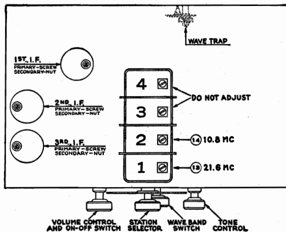
Fig. 2. Top View
