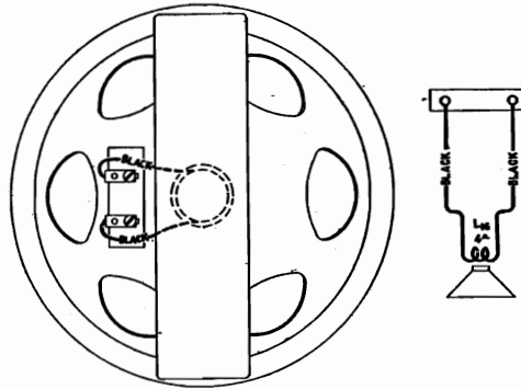
Figure 3—Loudspeaker Wiring
