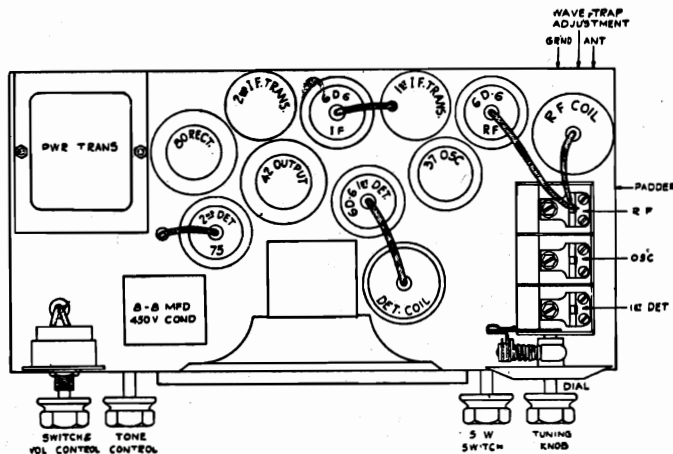
Tube Layout
