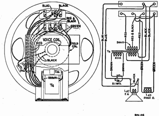
Figure 6—Loudspeaker Wiring
