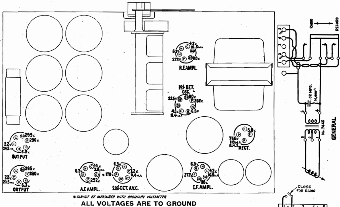
Figure 9—Universal Power Transformer Connections
