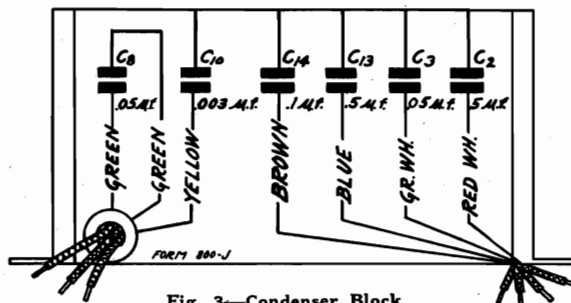
Fig. 3—Condenser Block.
