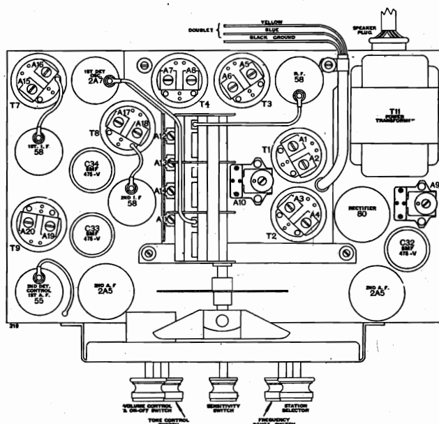
R. F. TRIMMERS ON MODELS 318 AND 447
