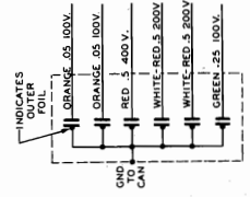
DIAGRAM OF BLOCK CONDENSER (B)
