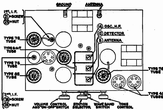
Fig. 2—Top View
