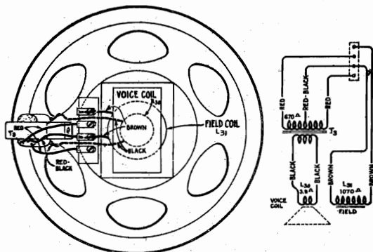
Figure 3—Console Loudspeaker Wiring
