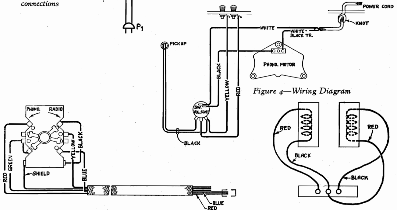
Figure 5—Cable Connections
