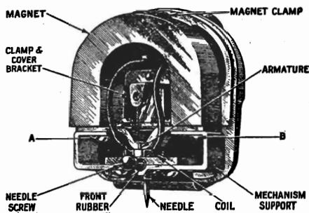
Figure 15—Pickup Nomenclature
