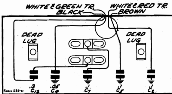
Condenser Block—Internal Wiring
