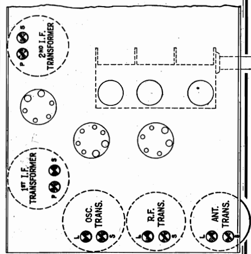
Figure 4—Location of Line-up Capacitors—Viewing bottom of chassis
