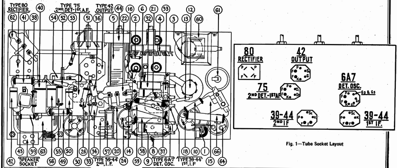
Fig. 4—Bottom View
