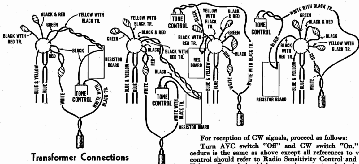
Figure F—Power Transformer Connections (50-60 cycles)
