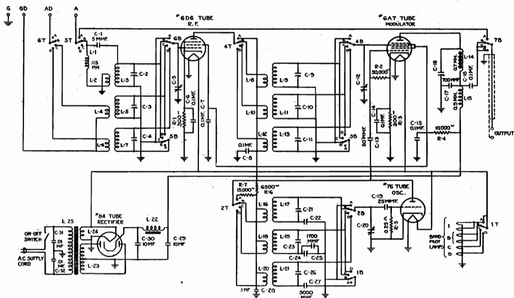
Fig. 1. Schematic Circuit
