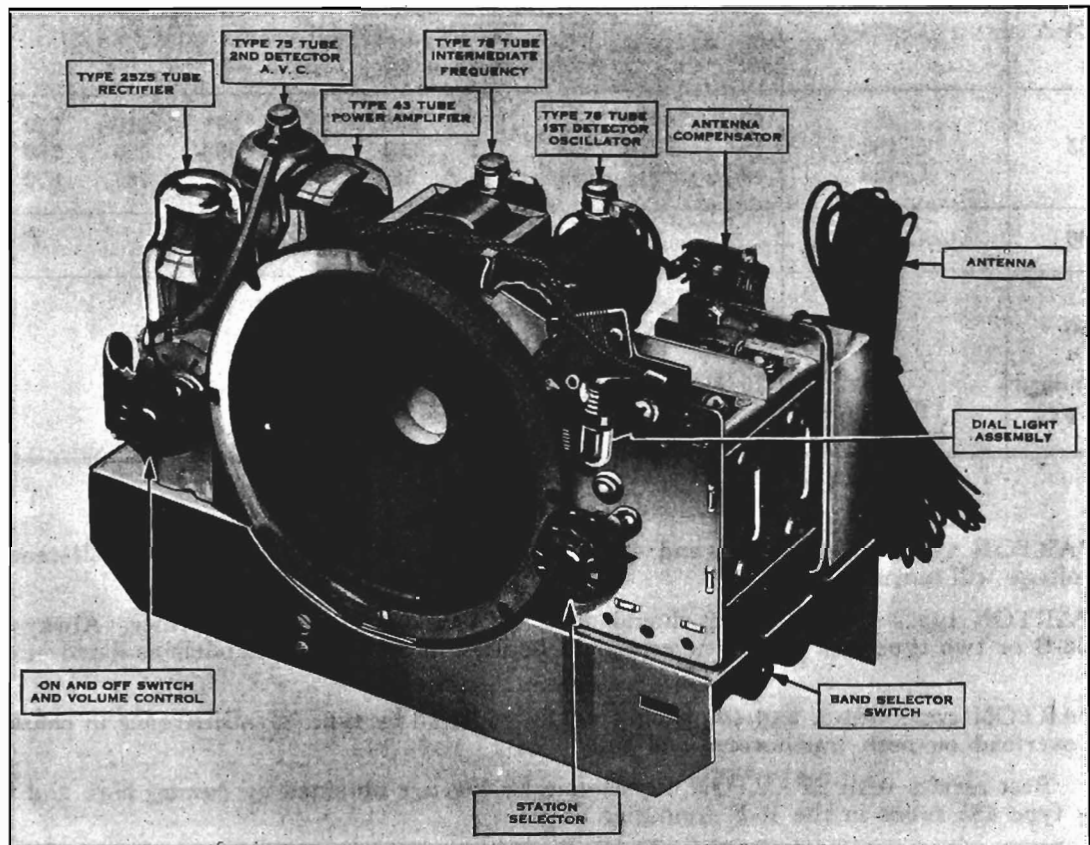
MODEL 57 CHASSIS
