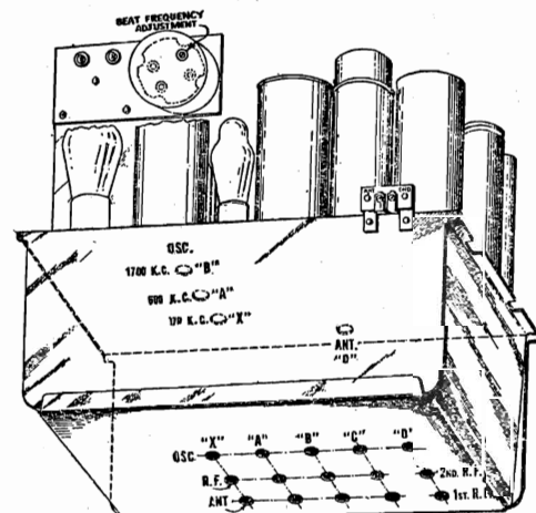
Figure E—Location of line-up capacitors.
