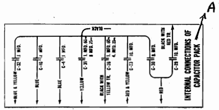
Figure A—Schematic Circuit
