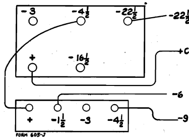
Fig. 3—Optional "C" Battery Connections
