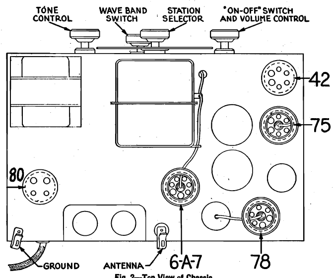
Fig. 2—Top View of Chassis
