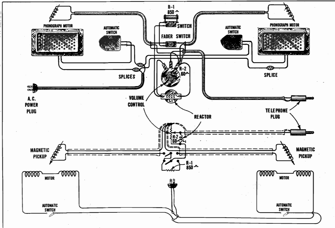
Figure C—Wiring and Schematic Diagrams (PT17A1, A2)
