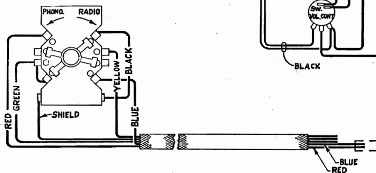
Figure 5—Cable Connections
