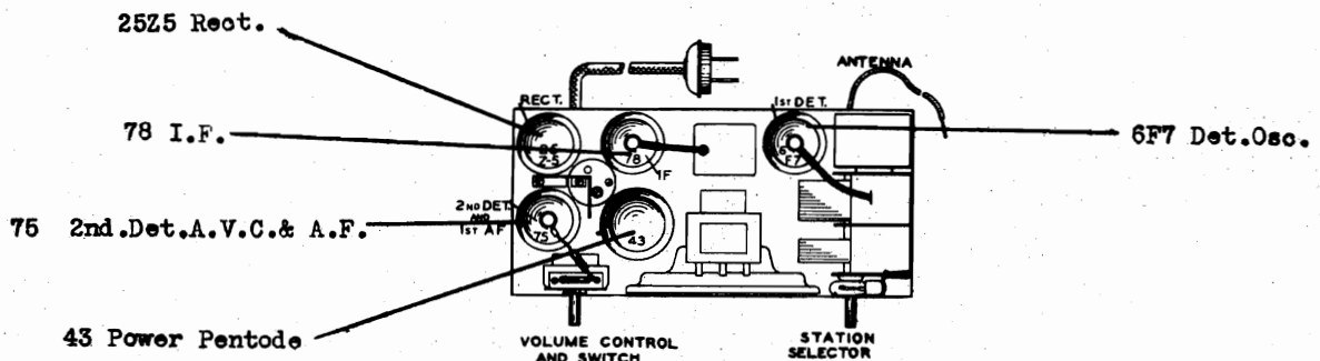
SCHEMATIC WIRING DIAGRAM MODEL 501
