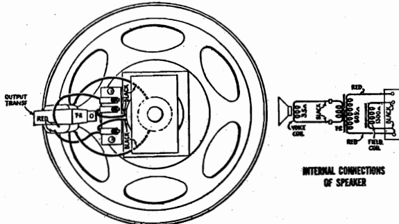
Figure C—Loudspeaker Wiring
