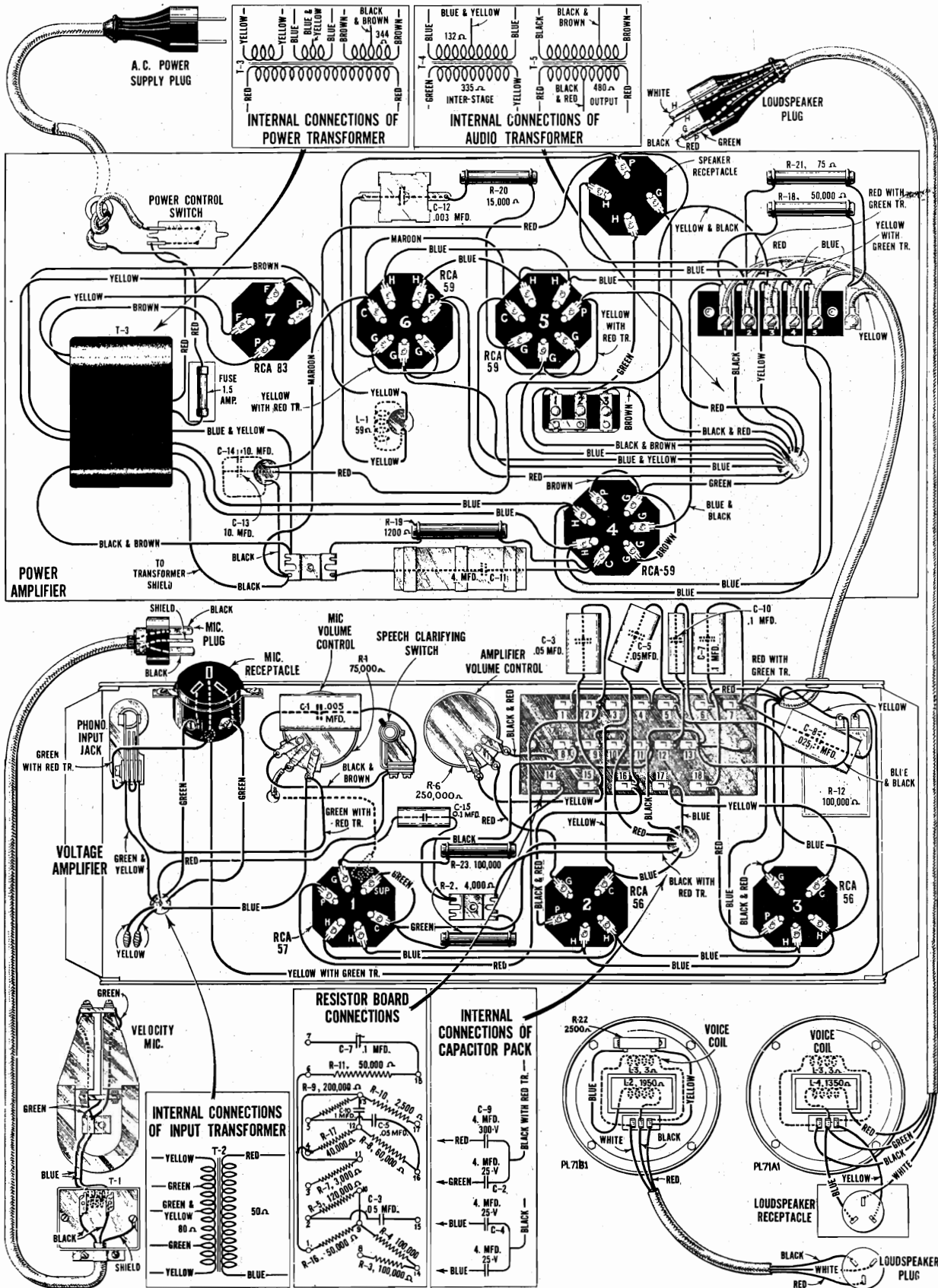
Figure 8—Wiring Diagram—PG-62 Equipment
