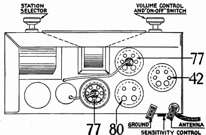
Fig. 2—Top View of Chassis
