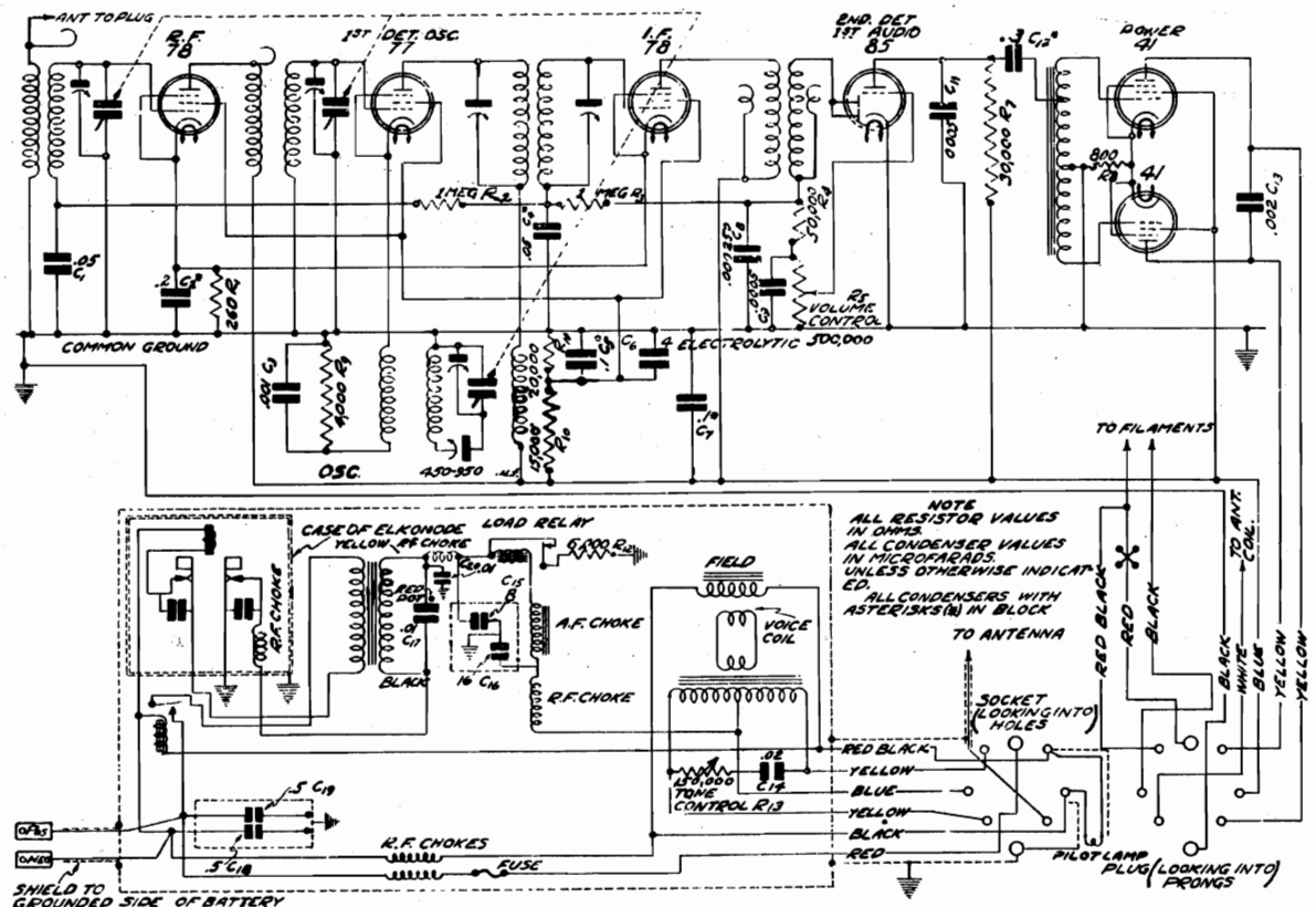
Fig. 9—Schematic Circuit Diagram
