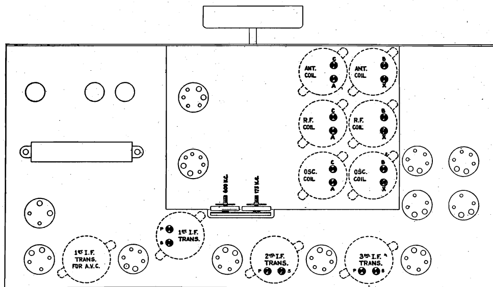
Figure 10—Location of Various Trimmer Capacitors
