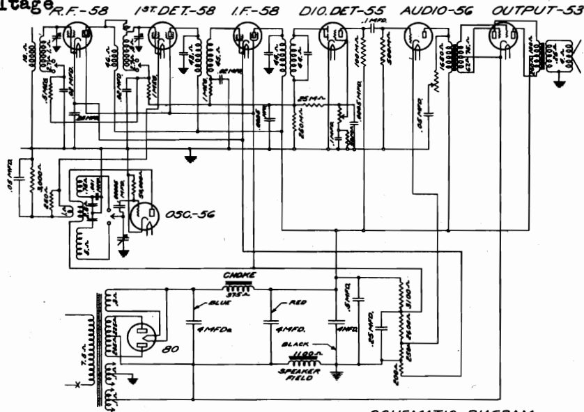
SCHEMATIC DIAGRAM OF MODEL 14-A DRAWN BY L.J. CHECKED BY APPROVED DATE - 11-8-33
