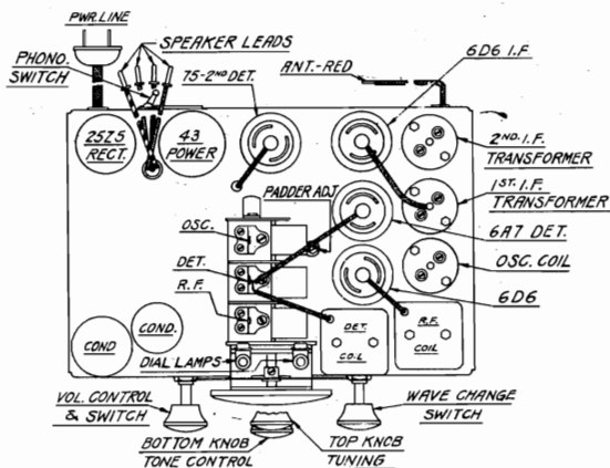
Tube Position
