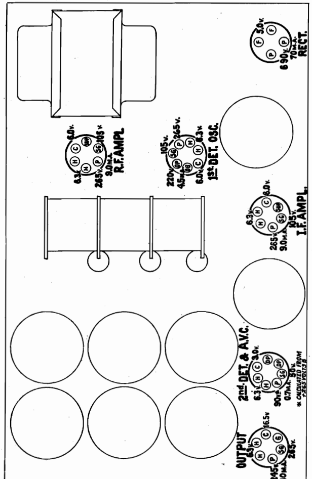
Figure 7—Tube Socket Voltages
