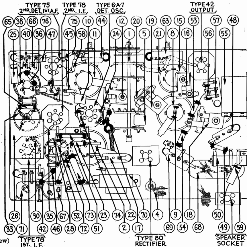
Fig. 1—Tube Sockets (underside)
