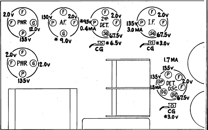
Figure 5—Socket Voltage Readings
