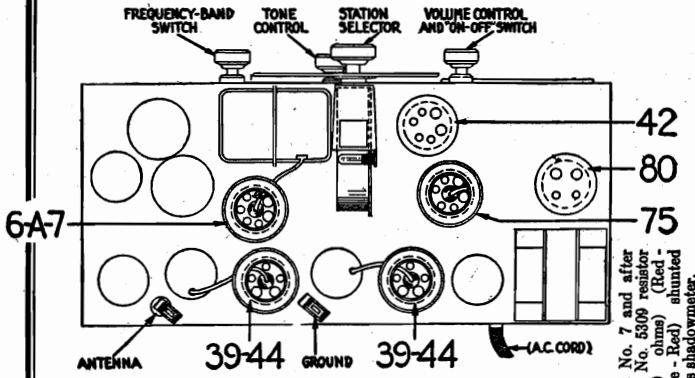
Fig. 2—Top View
