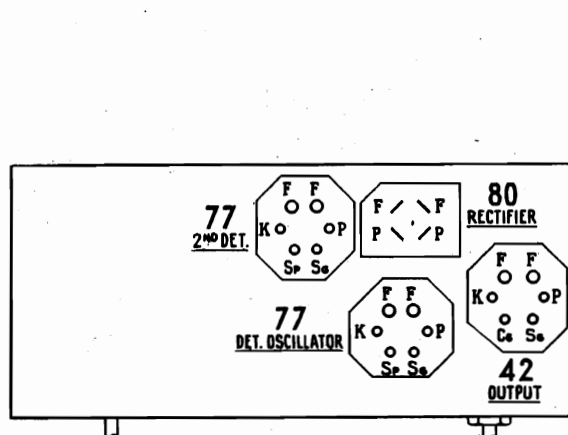
Fig. 1—Tube Socket Layout (Viewed from Bottom)
