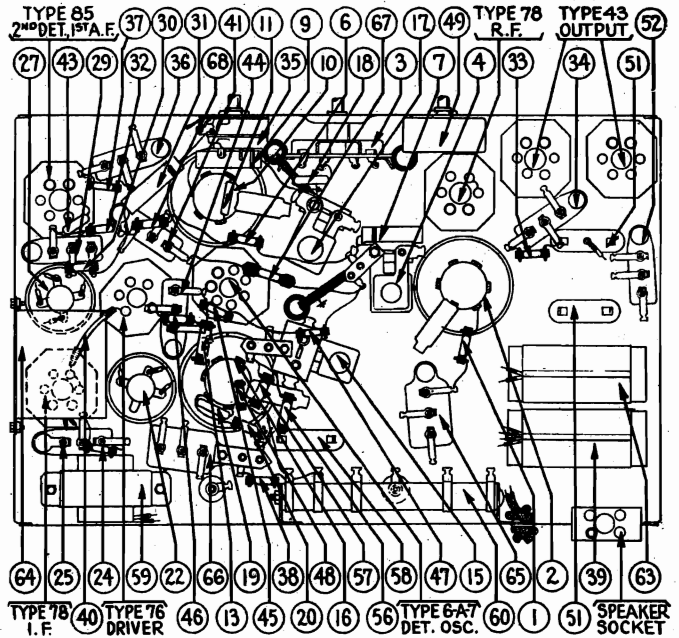
Fig. 4—Bottom View
