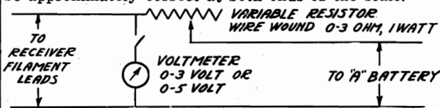
Fig. 4—Using Voltage Regulator with 3 Volt "A" Battery
