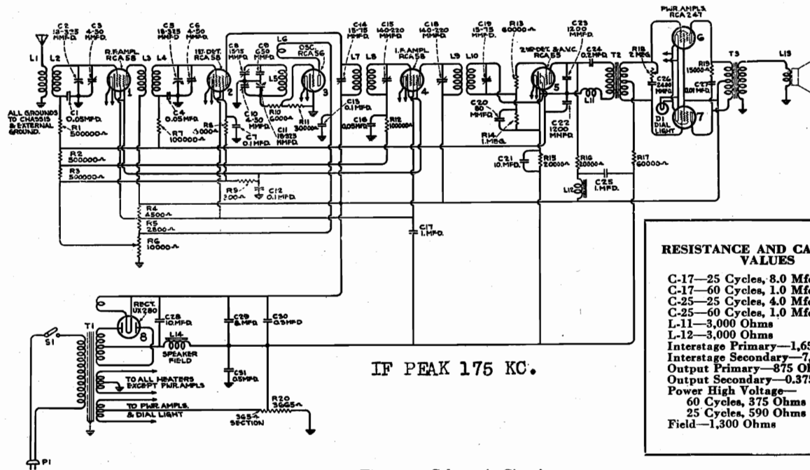
Figure 3—Schematic Circuit.
