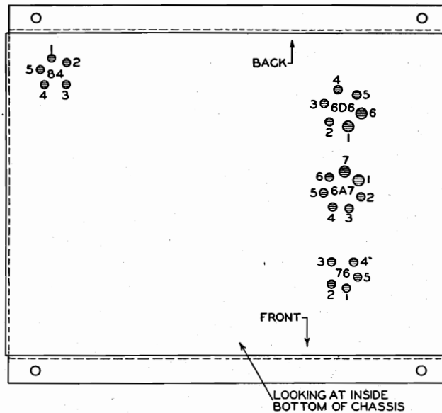
Fig. 2. Terminal Layout for Voltage Measurement Chart.
