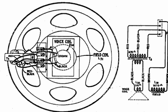
Figure 3—Loudspeaker Wiring
