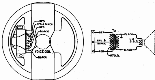
Figure 3—Loudspeaker Wiring
