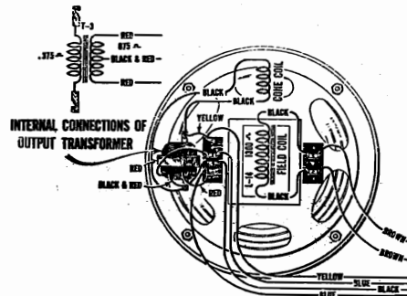
Figure 6—Loudspeaker Wiring
