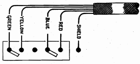
Junior "Duo" Connections
