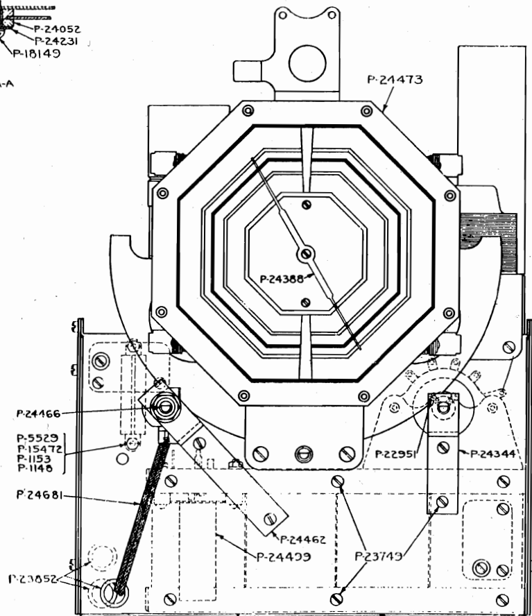
Fig. 4. Chassis Assembly.
