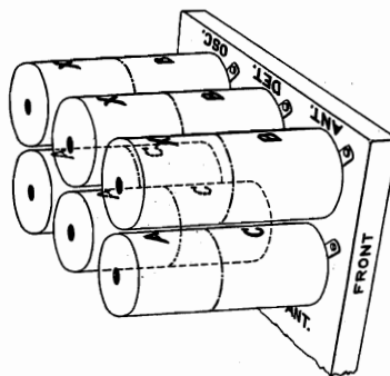
Figure 5—Location of Coils in Shields
