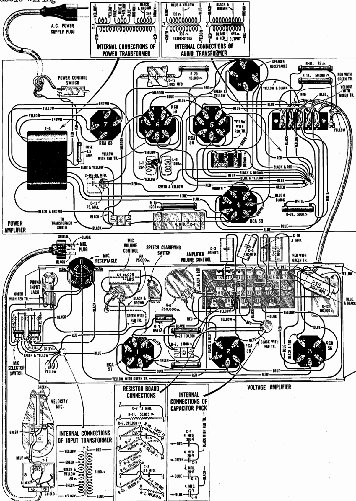
Figure 10—Wiring Diagram—Universal Amplifier
