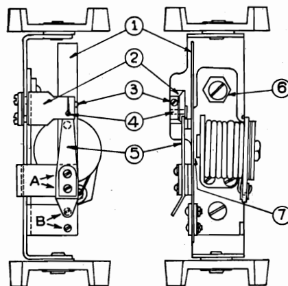
No. I 1. Reed Assembly 2. Stop Post mntg. block 3. Stop Post locking-screw 7. Air-gap No. II 4. Stop-Post 5. Contact Spring Assm. 6. Cam-nut adjustment
