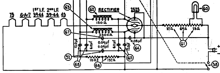
Fig. 3—Schematic Wiring Diagram
