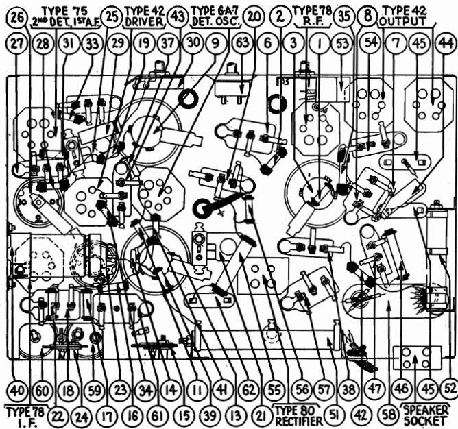
Fig. 4—Bottom View of Chassis Showing Parts
