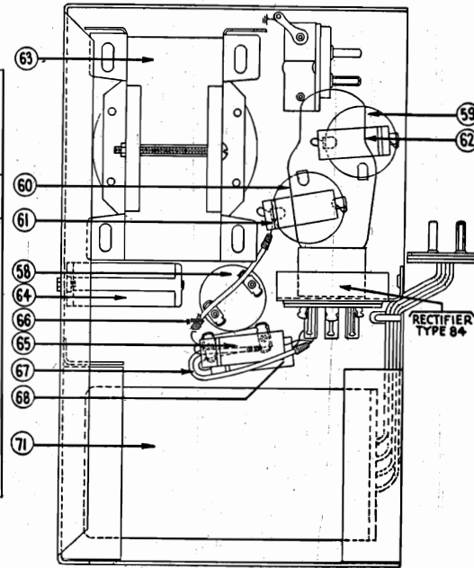
Fig. 7—Bottom of Vibrator and Rectifier Unit
