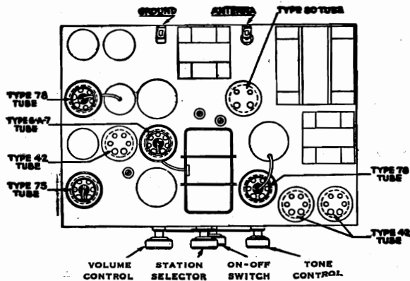
Fig. 2—Top View of Chassis
