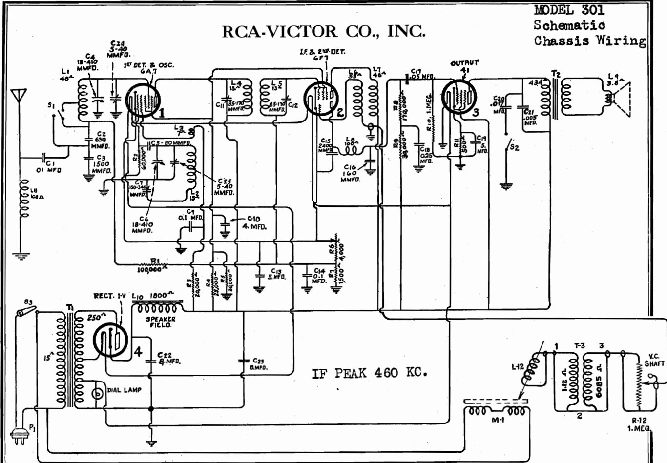
Figure C—Schematic Circuit Diagram
