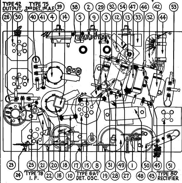
Fig. 4—Base View
