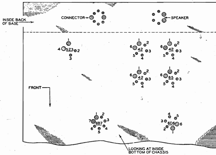
Fig. 1. Terminal Layout for Voltage Measurement Chart
