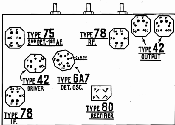
Fig. 1—Socket Layout (Underneath)
