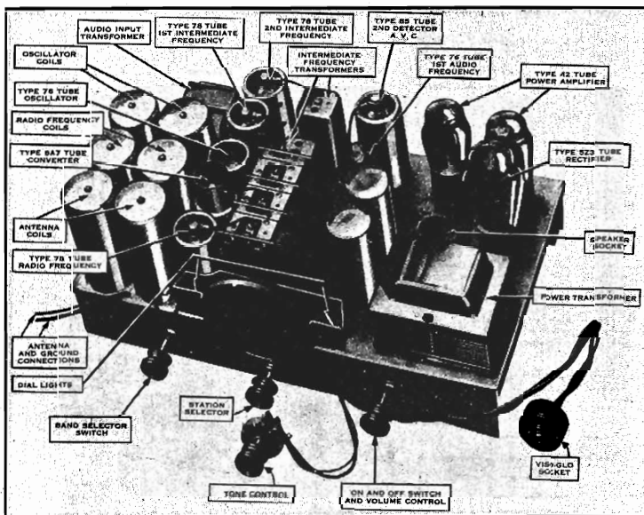
MODEL 104 CHASSIS
