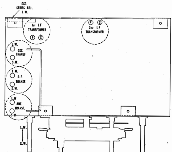
Figure E—Location of Line-Up Capacitors
