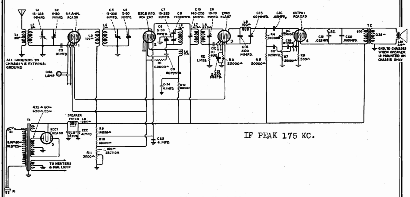
Figure 1—Schematic Circuit Diagram
