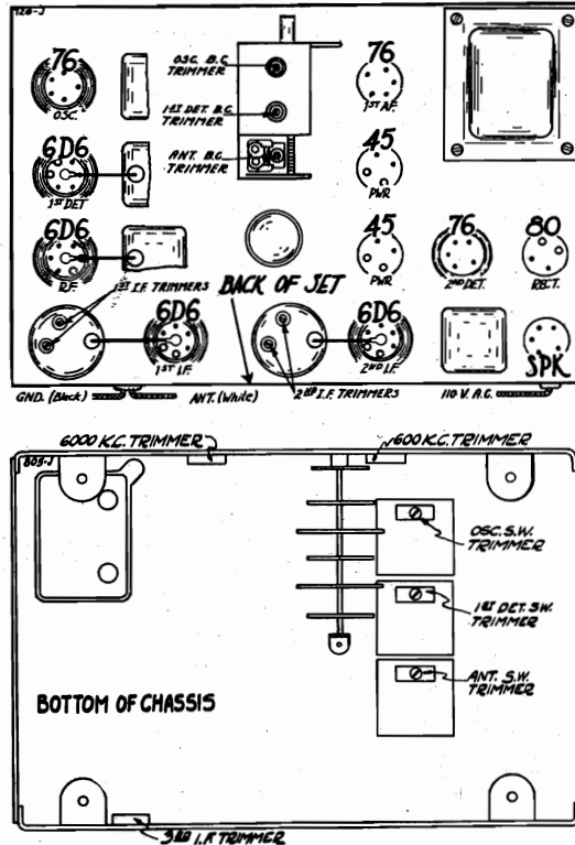
Fig. 2—Tube Arrangement & Location of Trimmers
