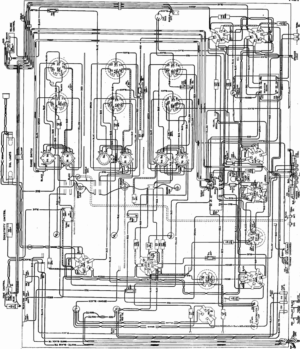
FIGURE 2 - CHASSIS WIRING
