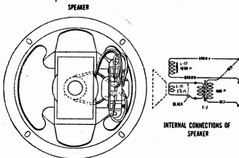
Figure C—Loudspeaker Wiring
