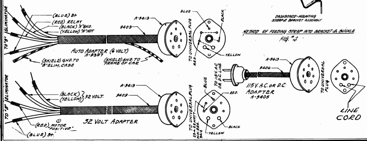
FIG. 2 SKETCH SHOWING CABLE CONNECTIONS TO 'B' ELIMINATOR OR 'B' BATTERIES FOR 6 VOLT A.C. OPERATION
