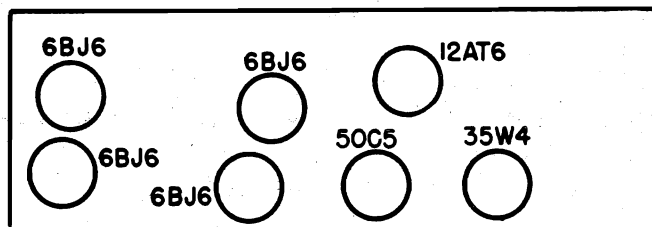
FIG. 2 TUBE LOCATION DIAGRAM FOR CHASSIS 120125-B
