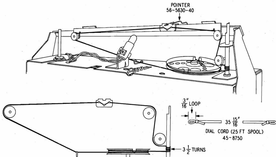
Figure 1. Drive-Cord Installation Details
