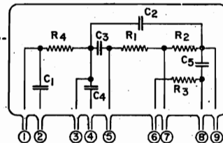
PC-165 WIRING DIAGRAM
