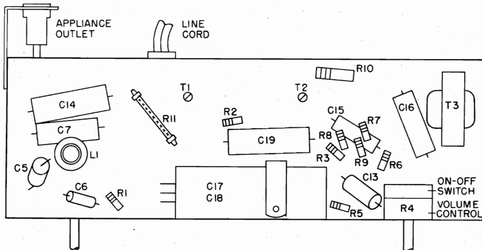
BOTTOM LAYOUT FOR 1-602-1 CHASSIS
