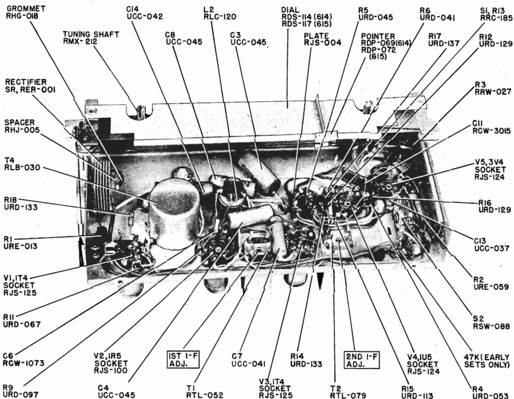
Components and Adjustments, Bottom View
