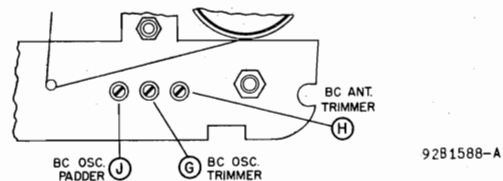
Fig. 6. Front View of Chassis Showing Location of Alignment Adjustments 92B1588-A
