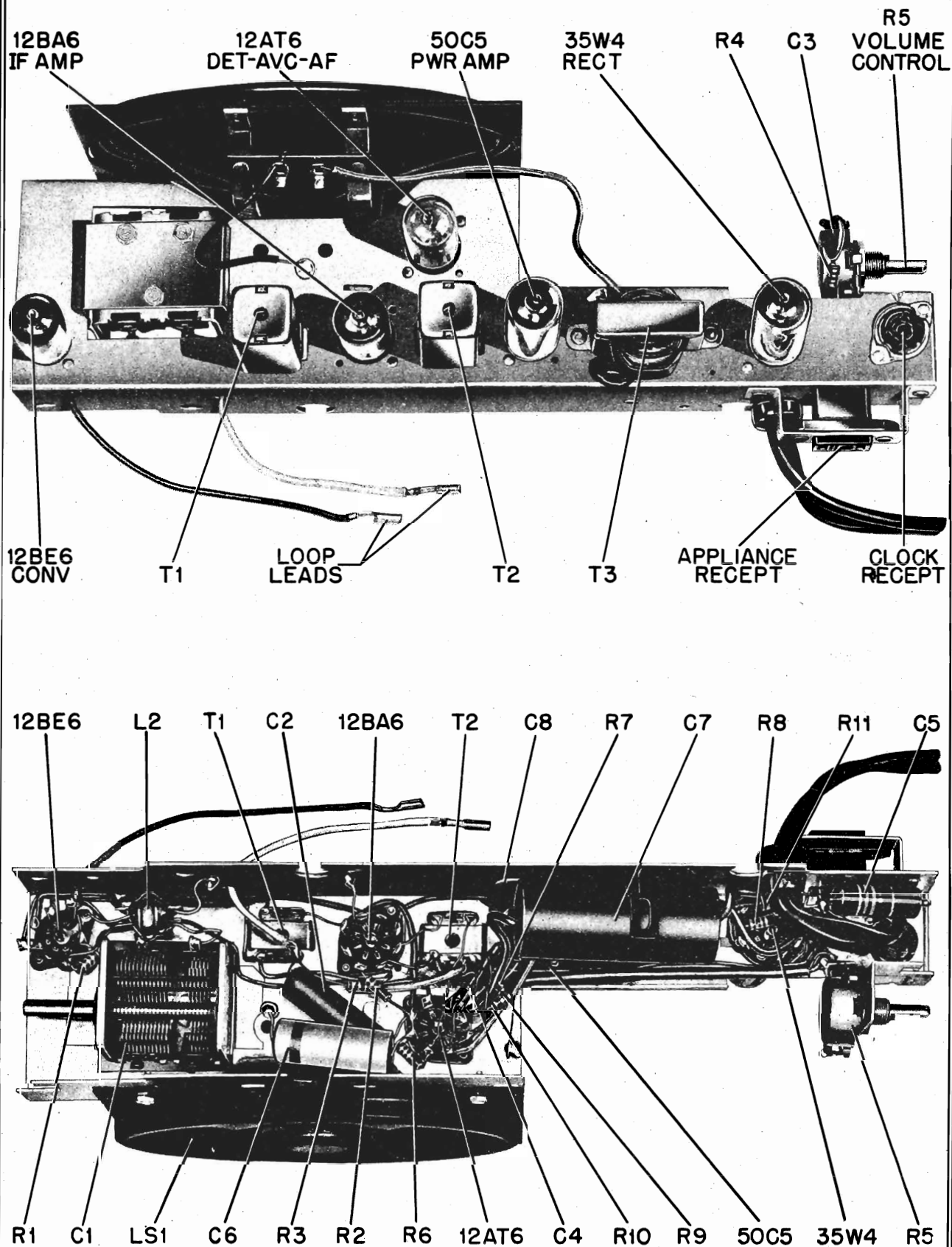
FIGURE 3. PARTS LOCATIONS
