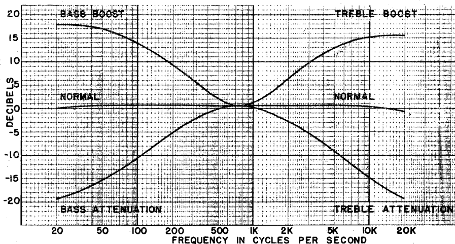
Fig. 2. Audio Characteristic
