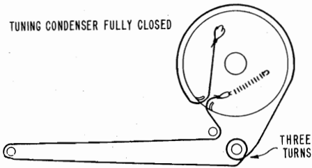
FIG. 5 - DIAL CORD DIAGRAM
