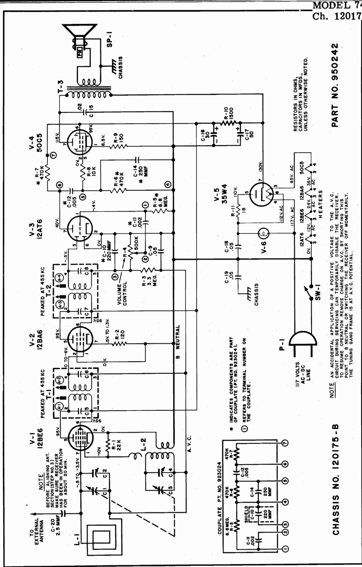
Fig. 1 - Schematic Diagram, Chassis 120175-B
