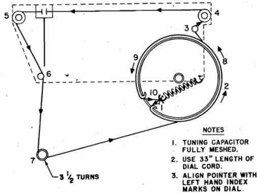
Fig. 4. Dial Cord Stringing Diagram 92C1569-A
