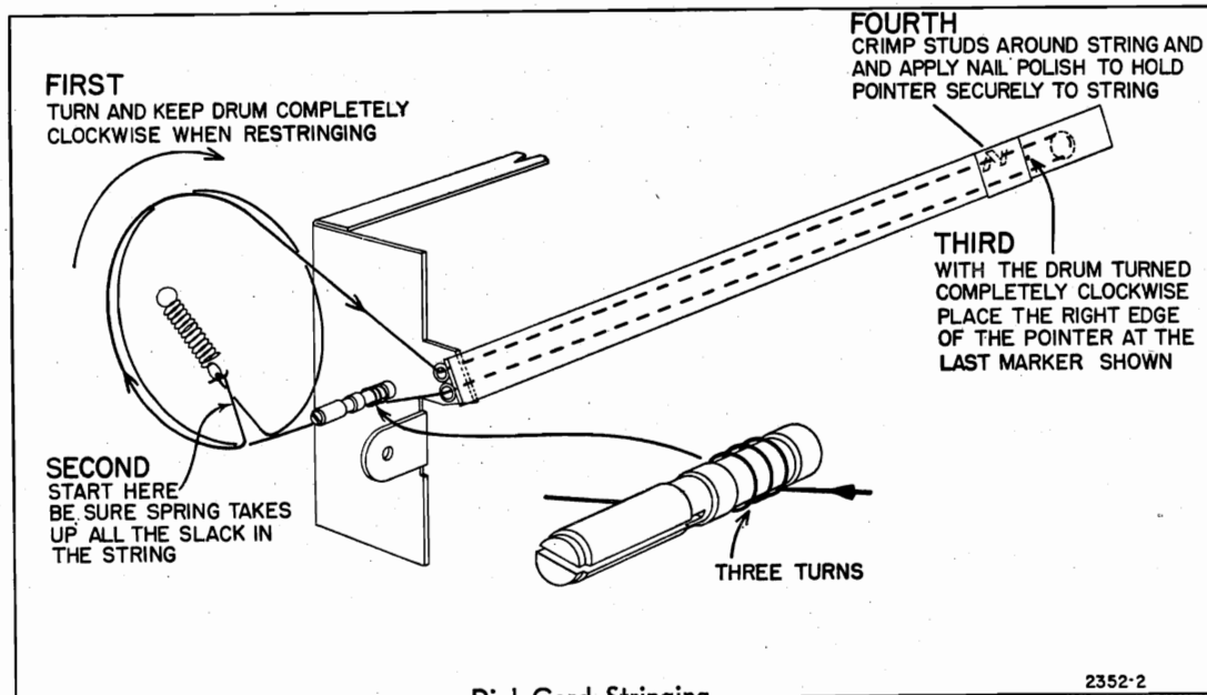
Dial Cord Stringing
