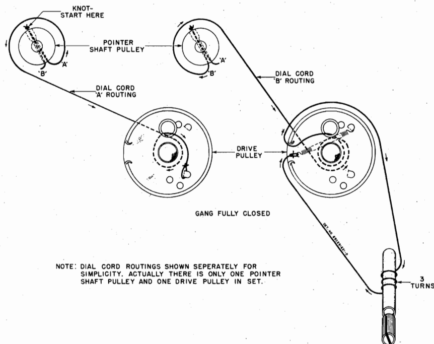
FIGURE 1. DIAL RESTRAINING DETAIL
