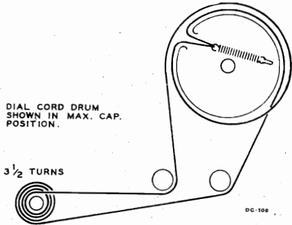
Dial Cord Drive
