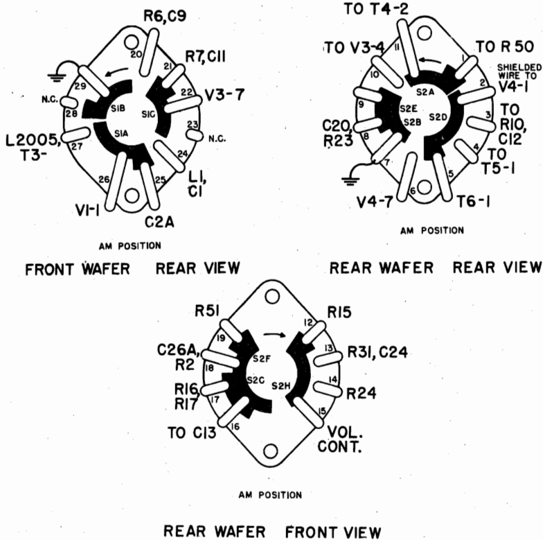
FIG. 7. SWITCH CONNECTIONS
