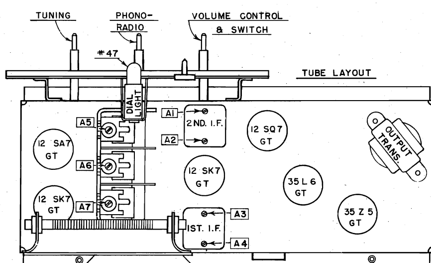
LOCATIONS OF PARTS UNDER CHASSIS
