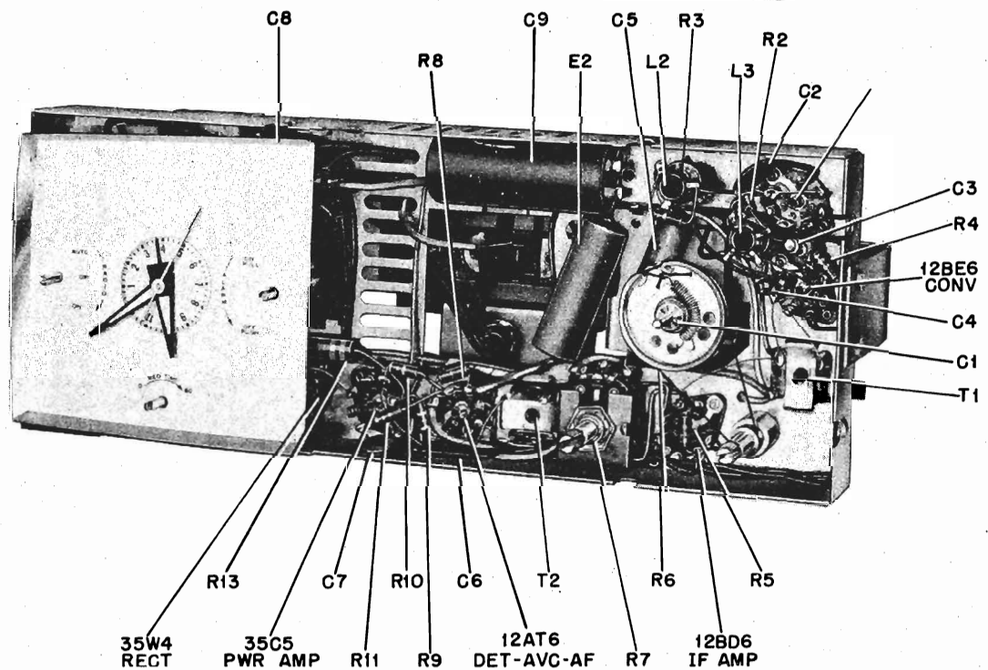
FIGURE 4. PARTS LOCATION
