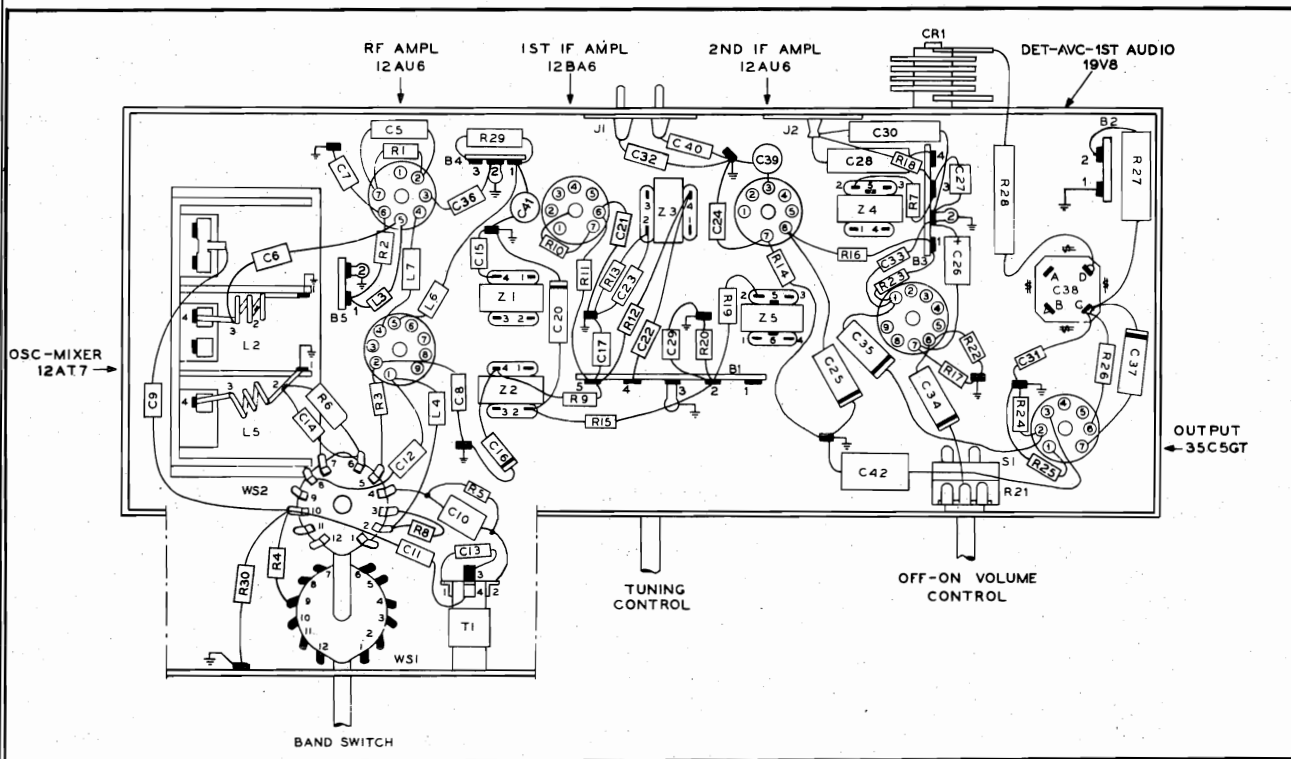
Figure 5. Base View, Showing Parts Placement
