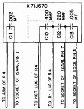
Couplate Unit, C10, 11, 12, 13
