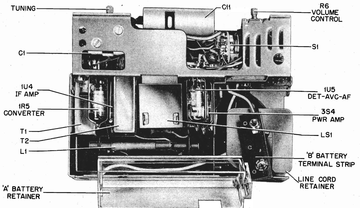
FIGURE 4. PARTS LOCATIONS
