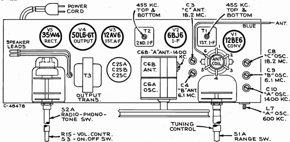
Tube and Trimmer Locations
