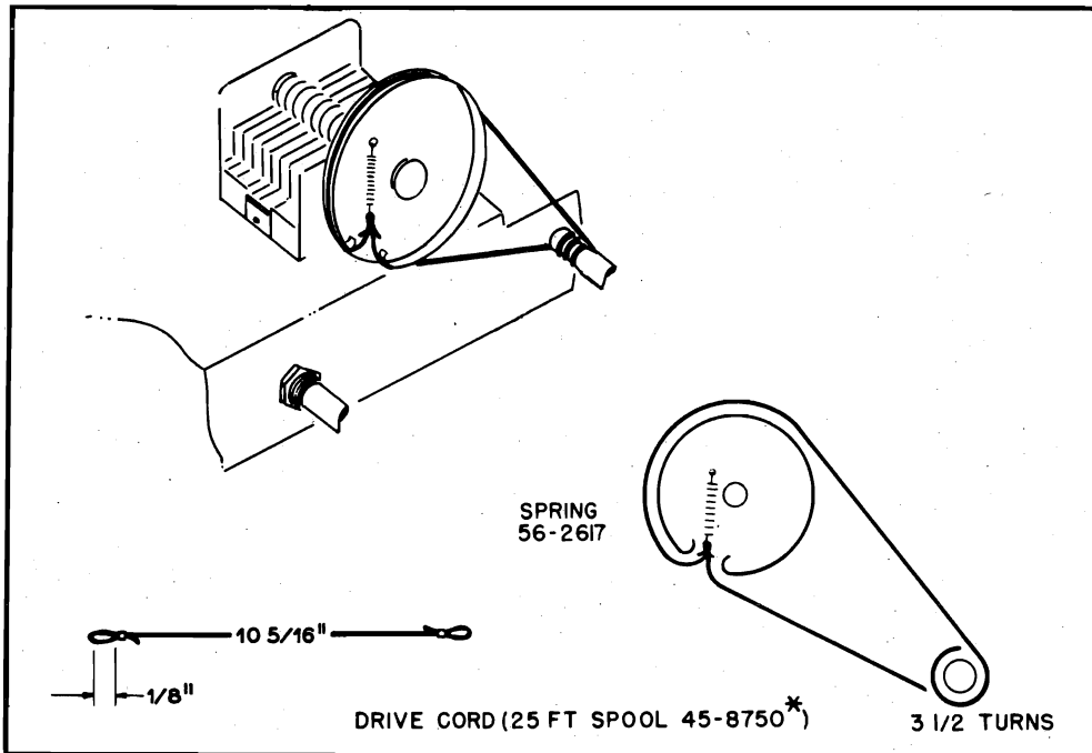
Figure 1. Dial-Cord Installation Details
