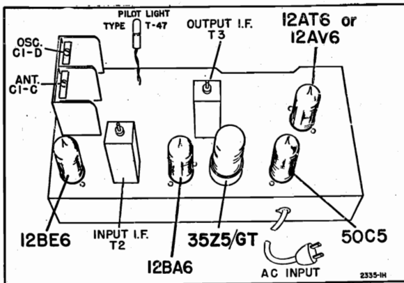
Chassis View
