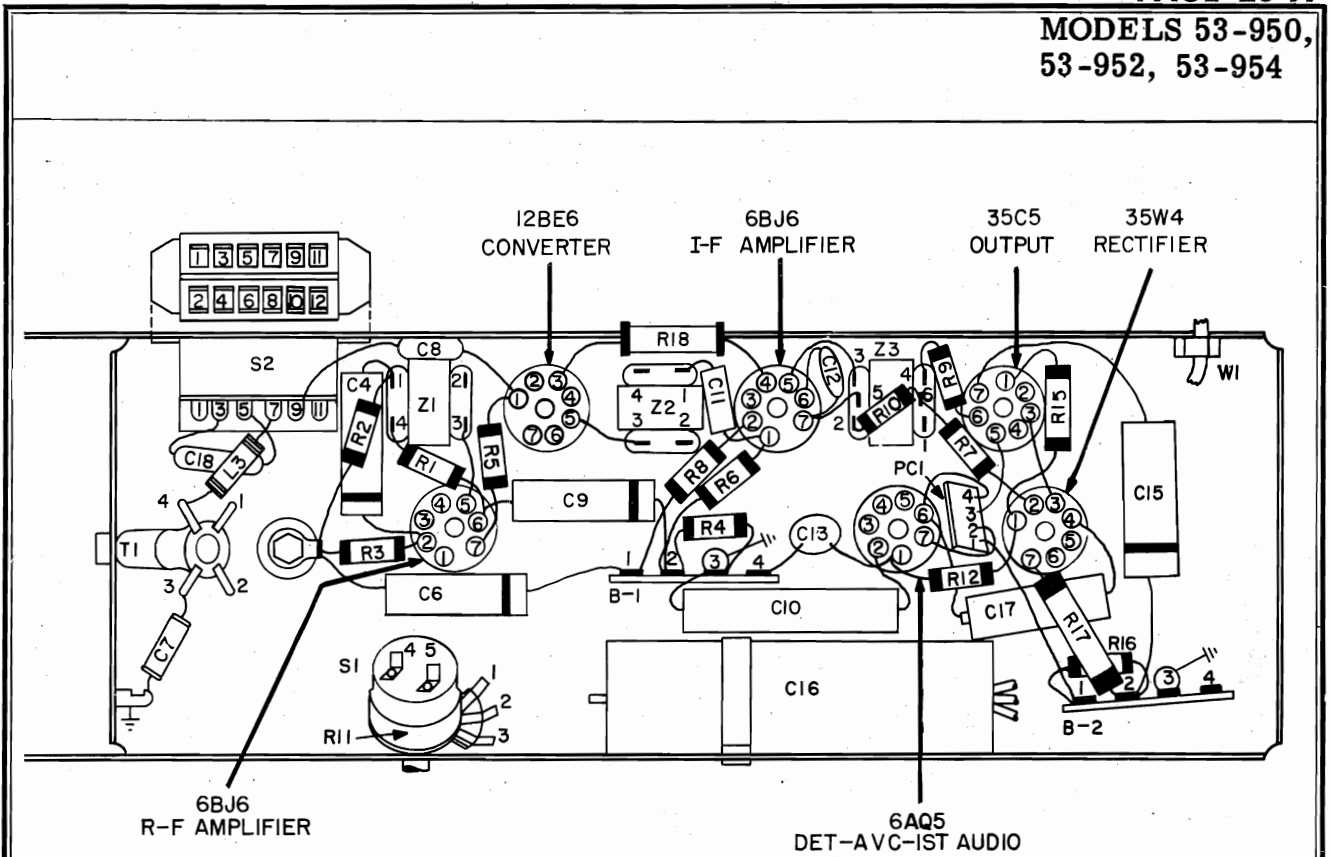
Figure 2. Top View, Showing Tuning Adjustments
