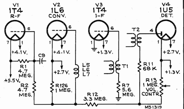
AVC Circuit
