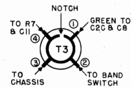
Fig. 8 COIL CONNECTIONS
