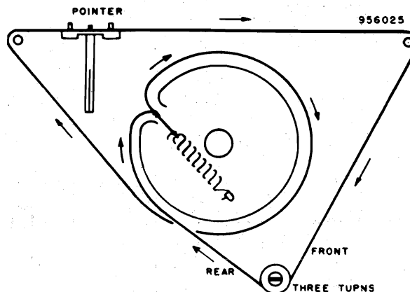
FIG. 3 DIAL CORD STRINGING FOR CHASSIS 120125-B
