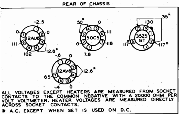
VOLTAGE TABLE (BOTTOM VIEW OF CHASSIS)
