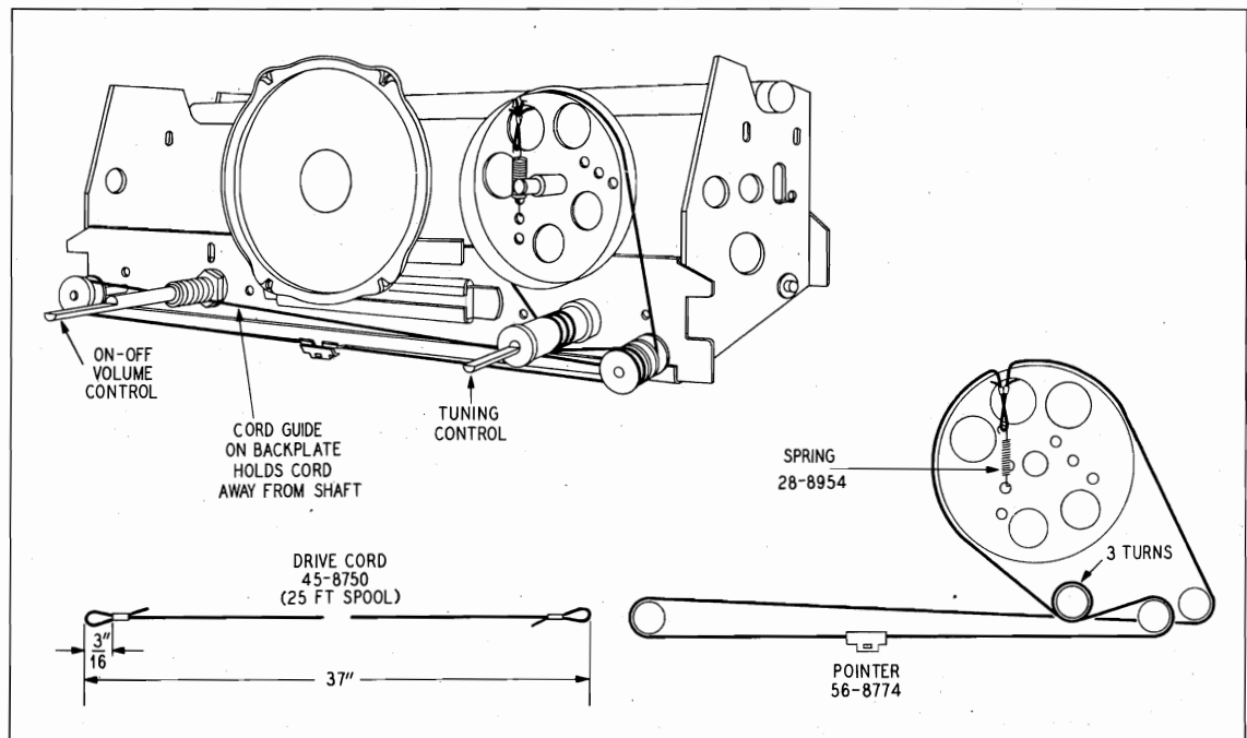
Figure 1. Drive-Cord-Installation Details
