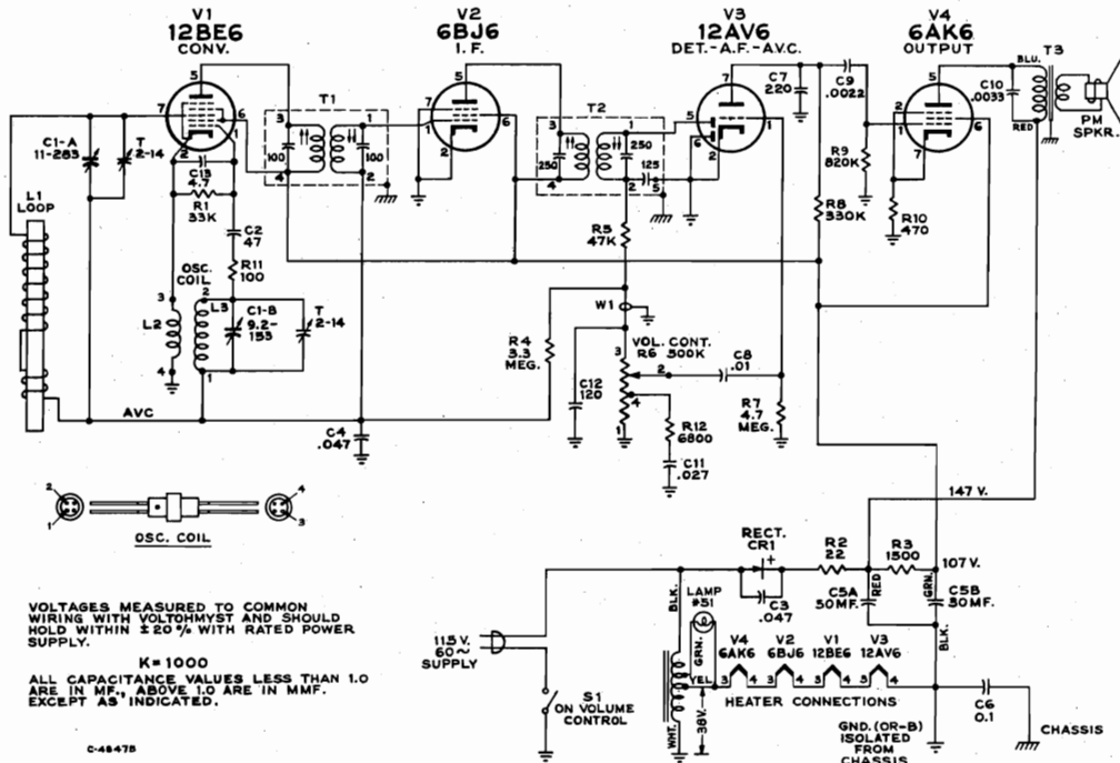
Schematic Diagram
