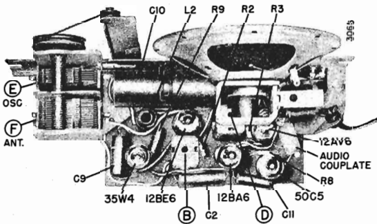
Figure 3. Top View of Chassis. Location of Components and Alignment Adjustments Shown. Adjustments A and C made from underside. See figures 1 and 2.
