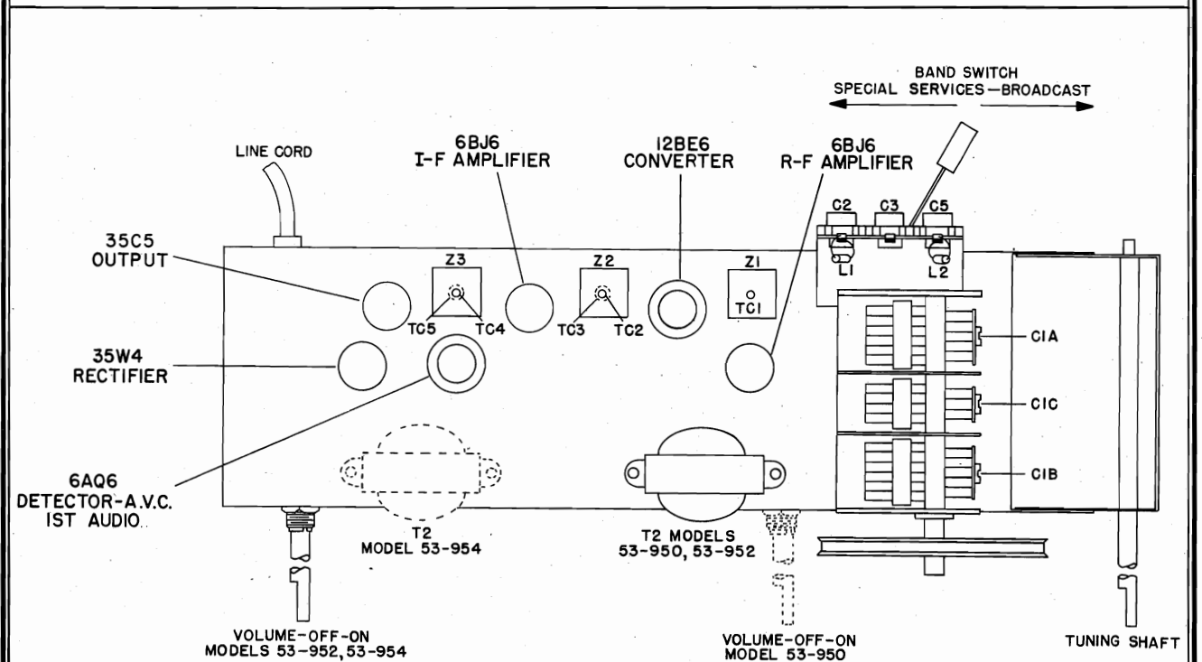
Figure 3. Base View, Model 53-950, Showing Parts Placement
