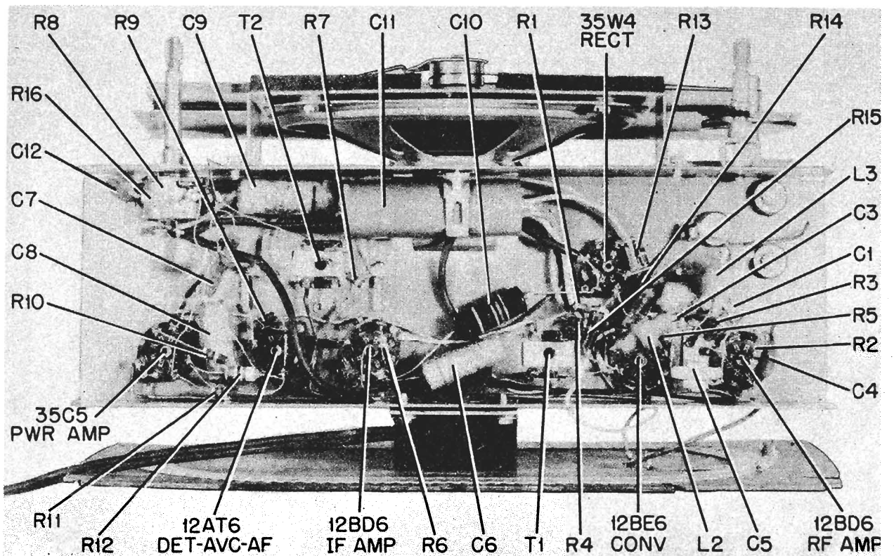
FIGURE 3. PARTS LOCATIONS
