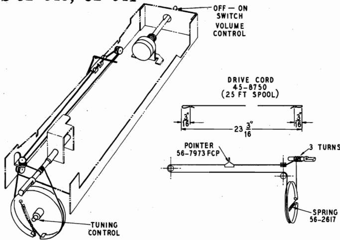
Figure 4. Drive-Cord-Installation Details
