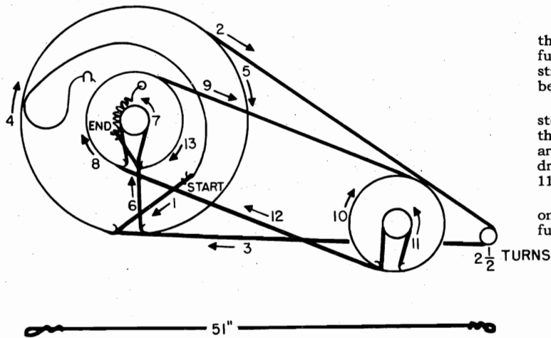
FIG. 5. DIAL STRINGING
