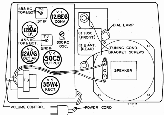
Tube and Trimmer Locations Chassis No. RC 1104C, RC 1104D, RC 1104E
