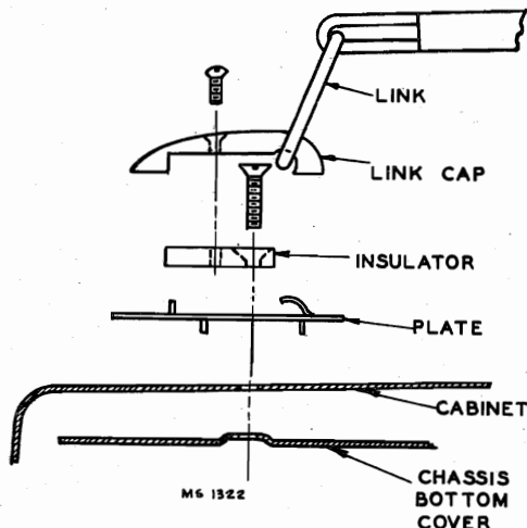
Chassis Mounting
