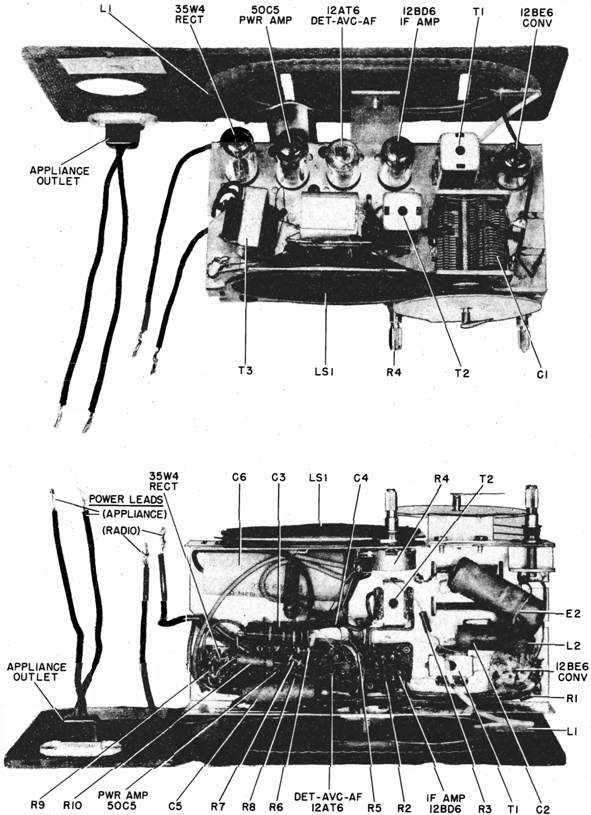
FIGURE 4. PARTS LOCATION
