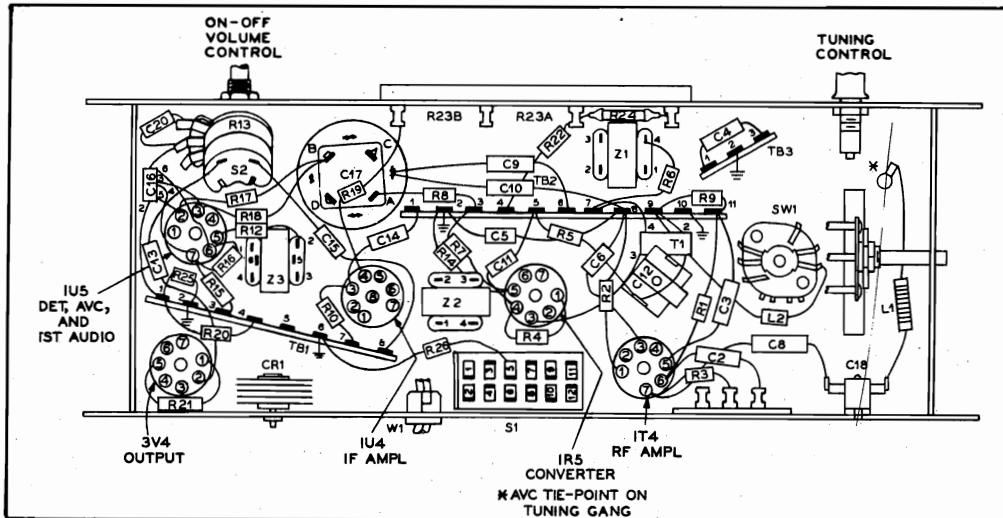
Figure 4. Bottom View, Showing Symbolized Chassis
