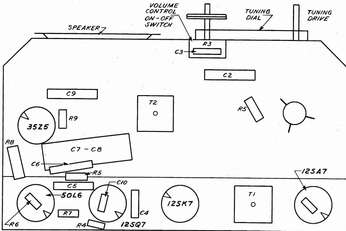
BOTTOM VIEW
