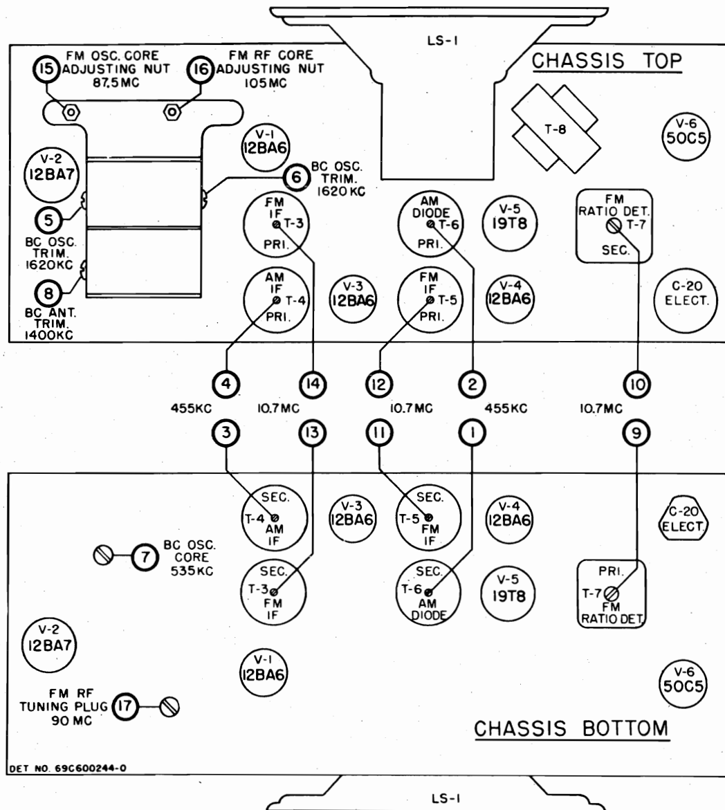
FIGURE 2. TUBE & TRIMMER LOCATIONS
