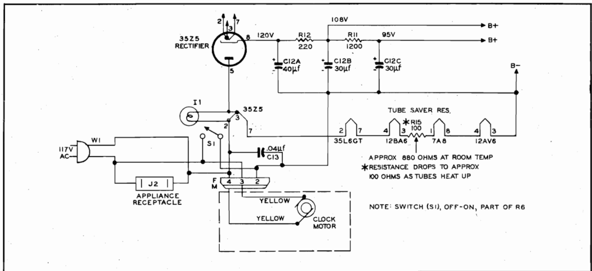
Figure 6. Model 52-543, Power and Clock Circuits TP2-1337
