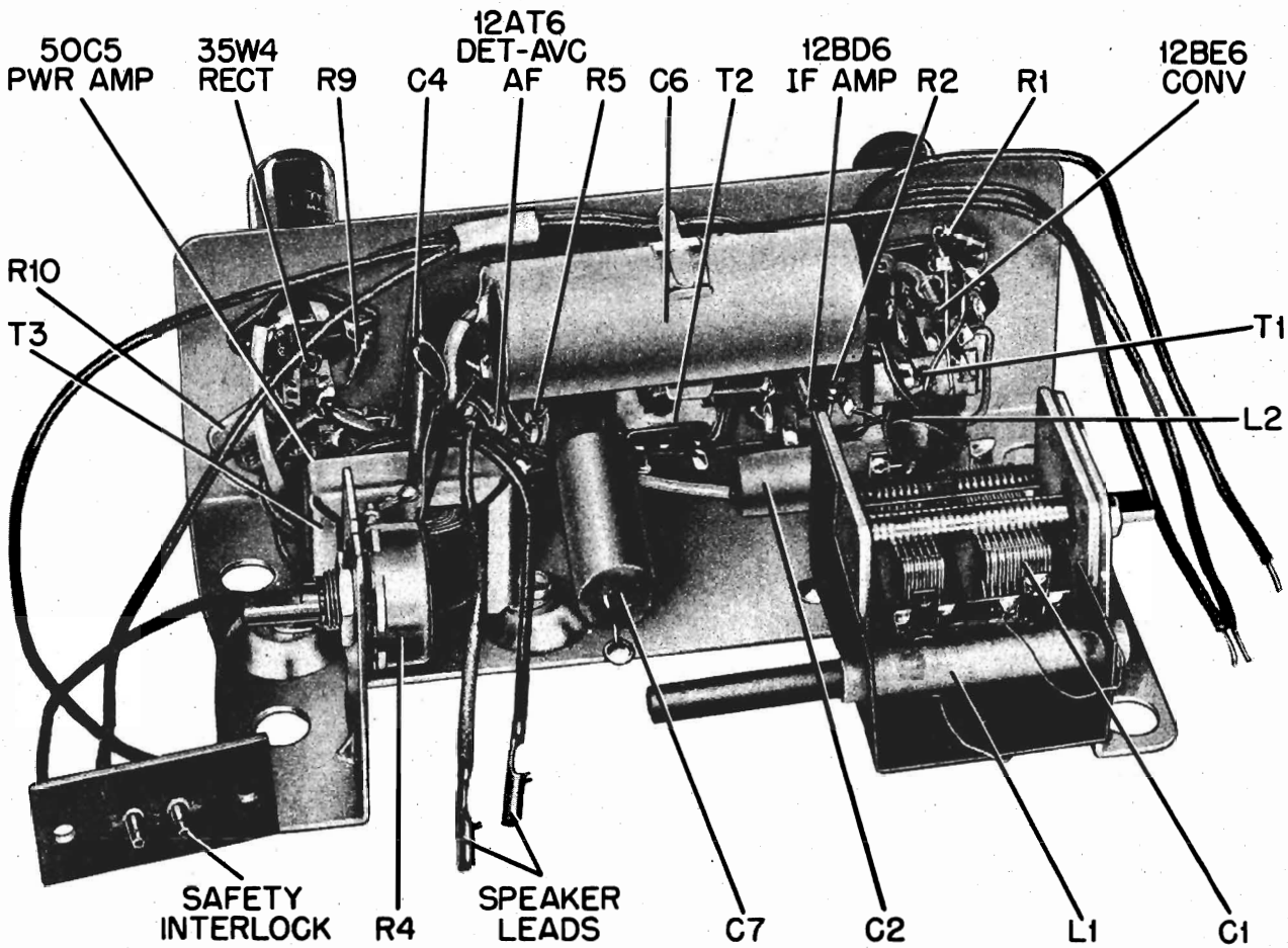
FIGURE 5. PARTS LOCATIONS
