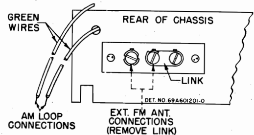
FIGURE 1. ANTENNA CONNECTIONS
