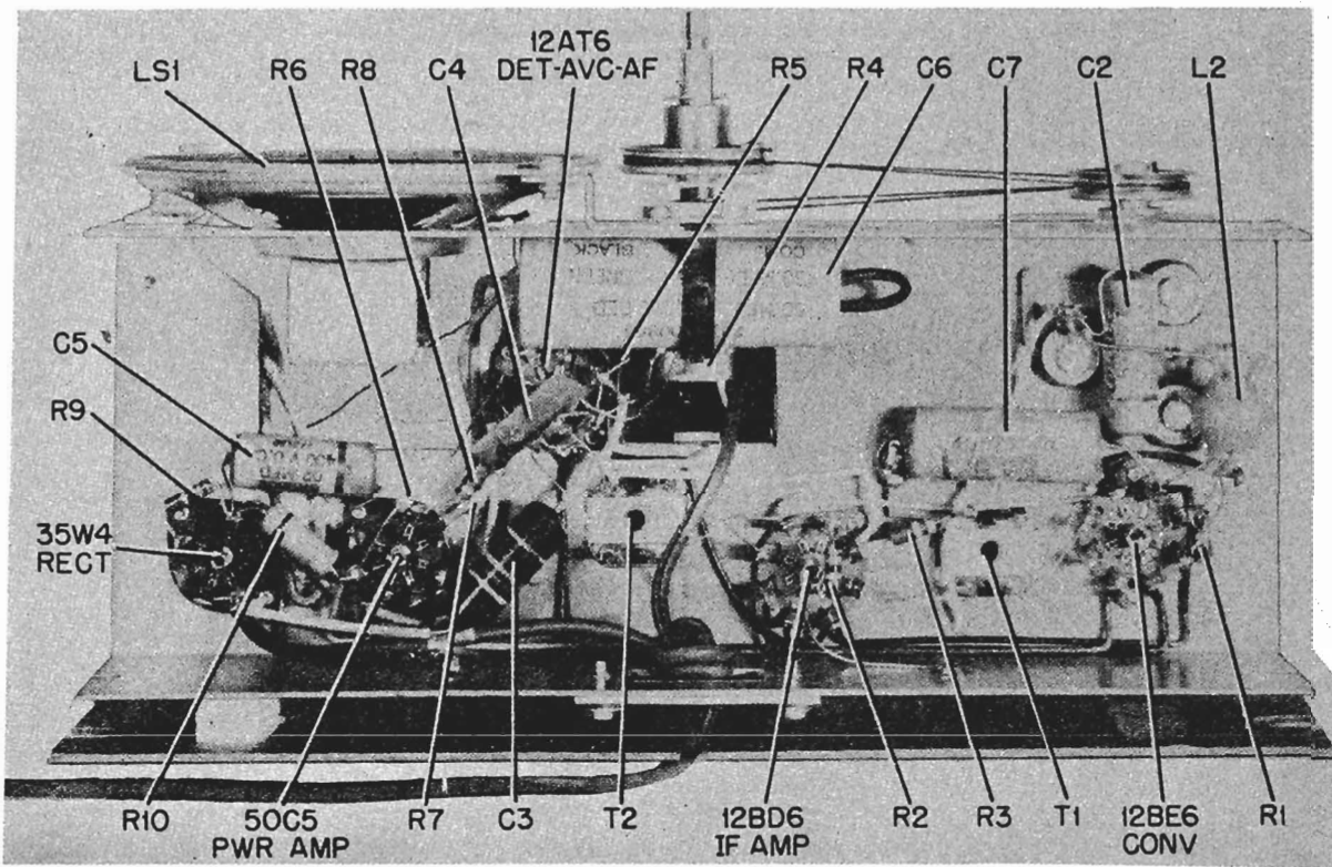
FIGURE 3. PARTS LOCATIONS
