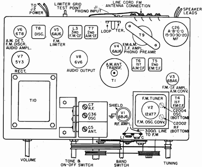
FIG. 1. TOP VIEW
