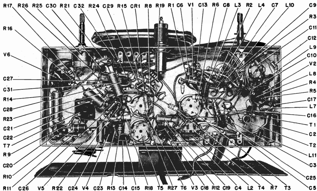
FIGURE 5. PARTS LOCATIONS
