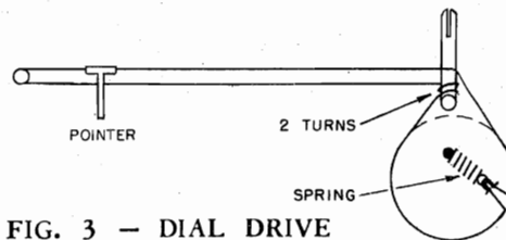
FIG. 3 - DIAL DRIVE
