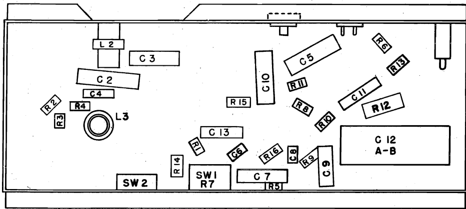
LOCATIONS OF PARTS UNDER CHASSIS
