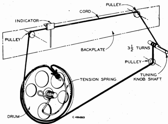
Dial Cord Layout
