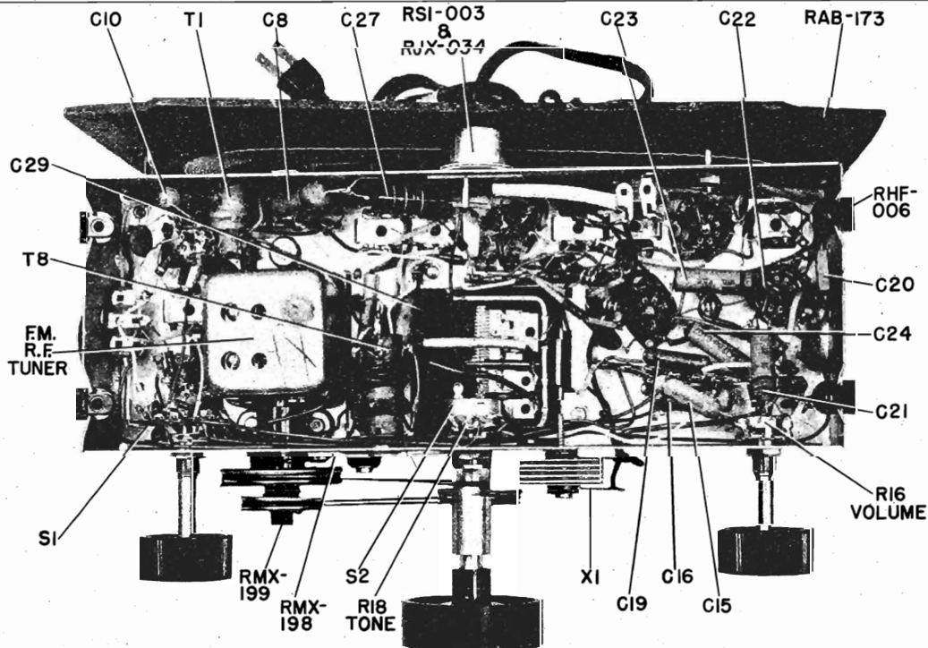
Fig. 6. BOTTOM VIEW
