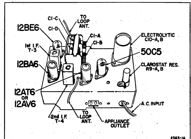
Chassis View
