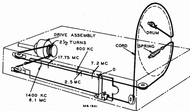
Dial Indicator and Drive Mechanism
