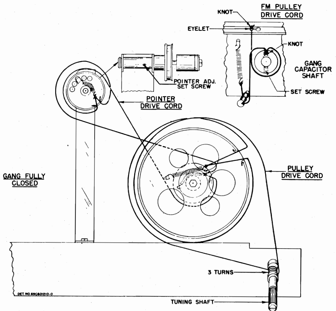
FIGURE 3. POINTER AND DRIVE CORD RESTRINGING DETAIL
