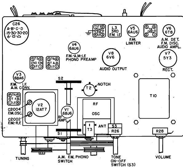
FIG. 2. BOTTOM VIEW
