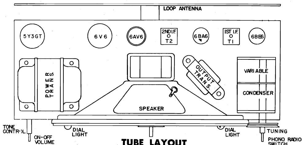
TUBE LAYOUT
