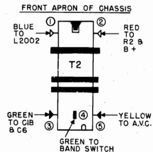
R.F. TRANSF. CONNECTIONS
