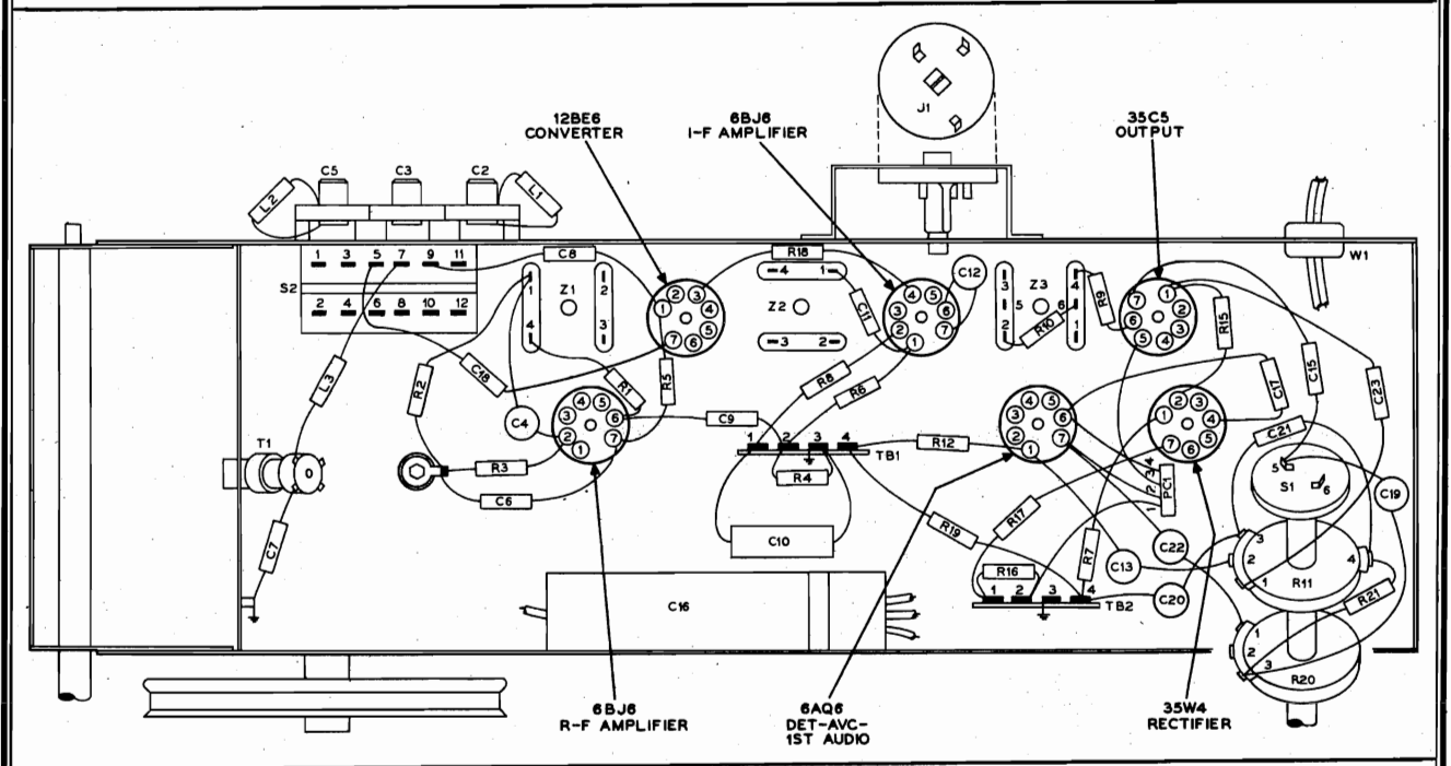
Figure 3. Base View, Showing Parts Placement
