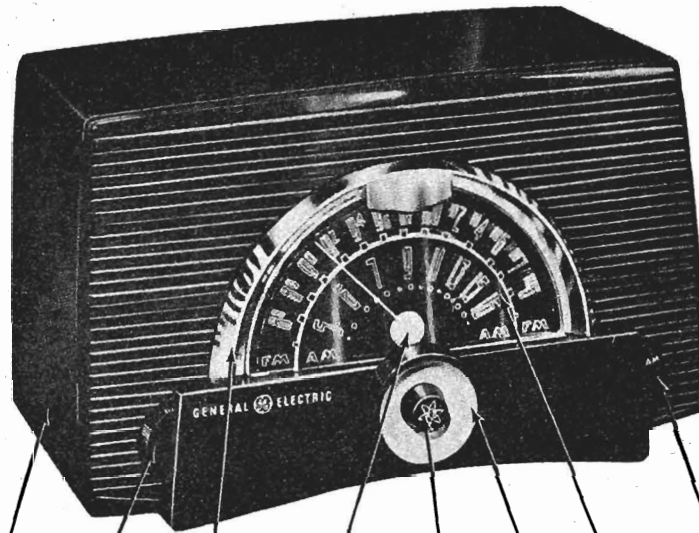
CABINET RAU-355 VOLUME RDK-211 ESCUTCHEON RDE-080 POINTER RDP-065 TONE RDK-266 TUNING RDK-265 DIAL RDS-111 BAND SWITCH RDK-267
