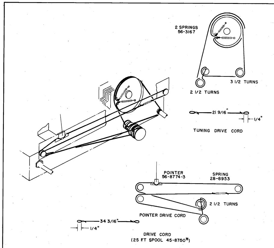
Figure 1. Dial-Cord Installation Details
