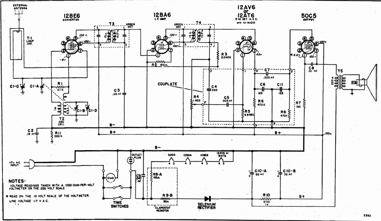
SCHEMATIC DIAGRAM
