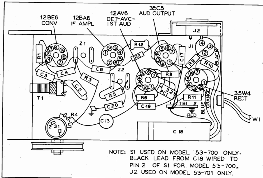
Figure 1. Base View, Showing Symbolized Chassis
