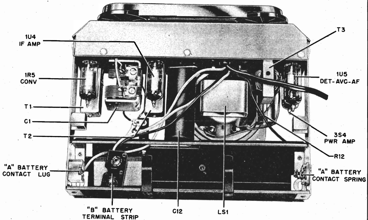
FIGURE 5. PARTS LOCATIONS
