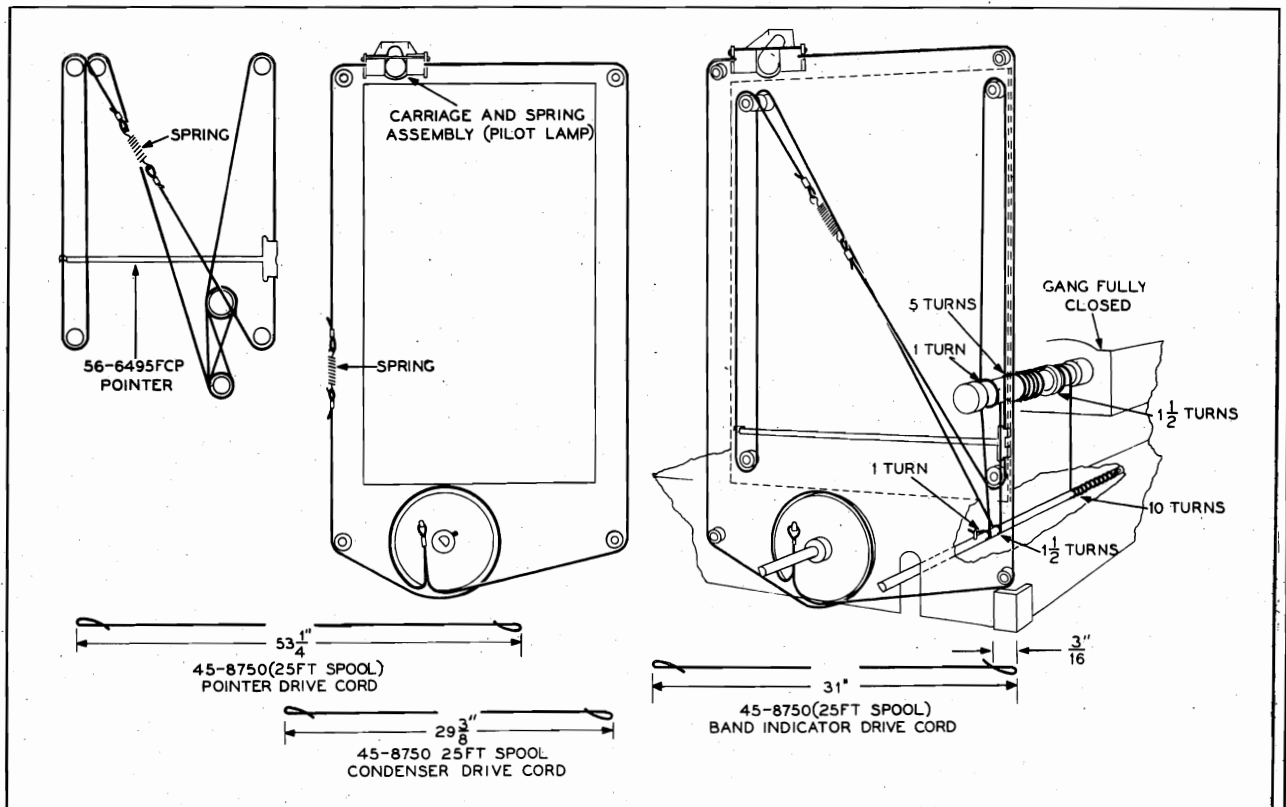
Figure 1. Drive-Cord Installation Details
