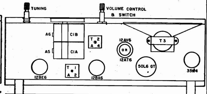
LOCATION OF TUBES AND TRIMMERS
