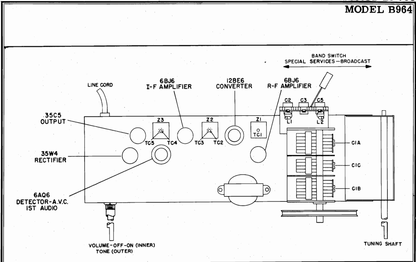
Figure 2. Top View, Showing Tuning Adjustments
