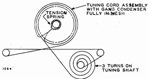
DIAL STRINGING
