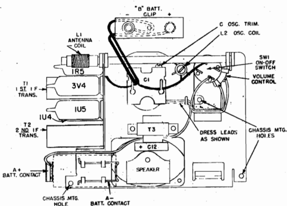
FIG. 2 – REAR VIEW OF V-2182-2 CHASSIS
