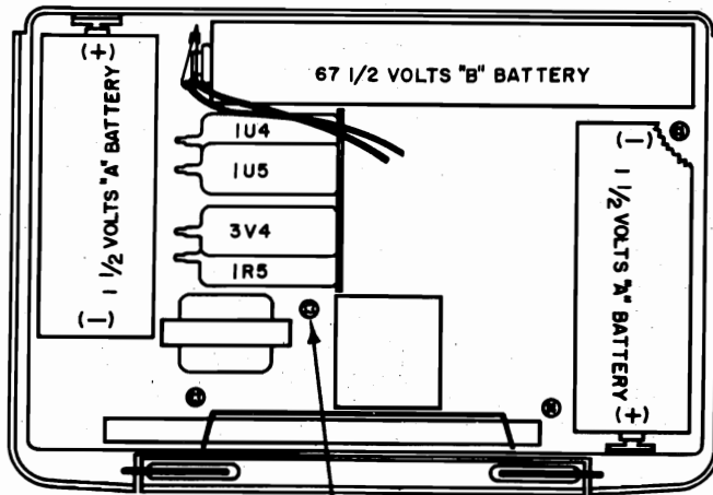
CHASSIS MOUNTING SCREWS (4) BATTERY & TUBE LOCATIONS 955375
