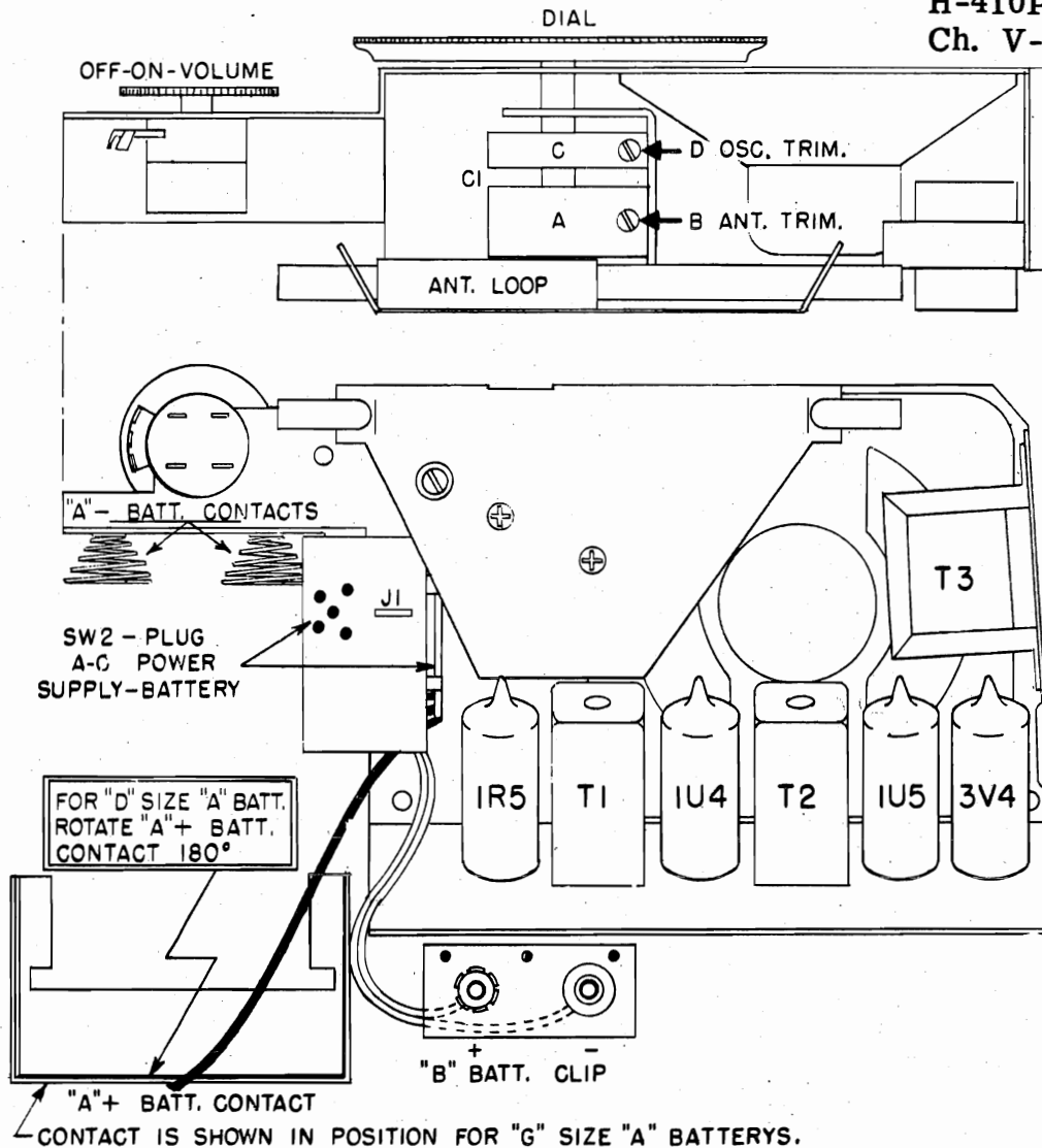
REAR VIEW OF V-2185-1 CHASSIS
