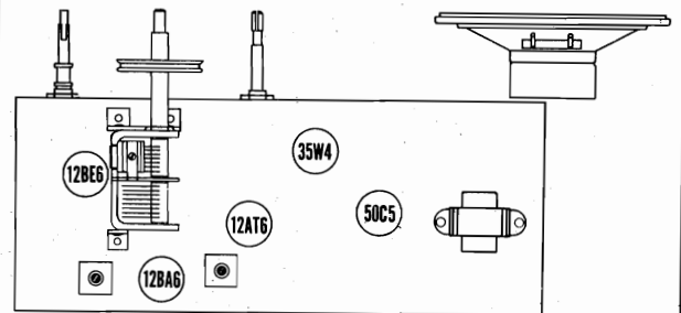
TUBE LOCATIONS
